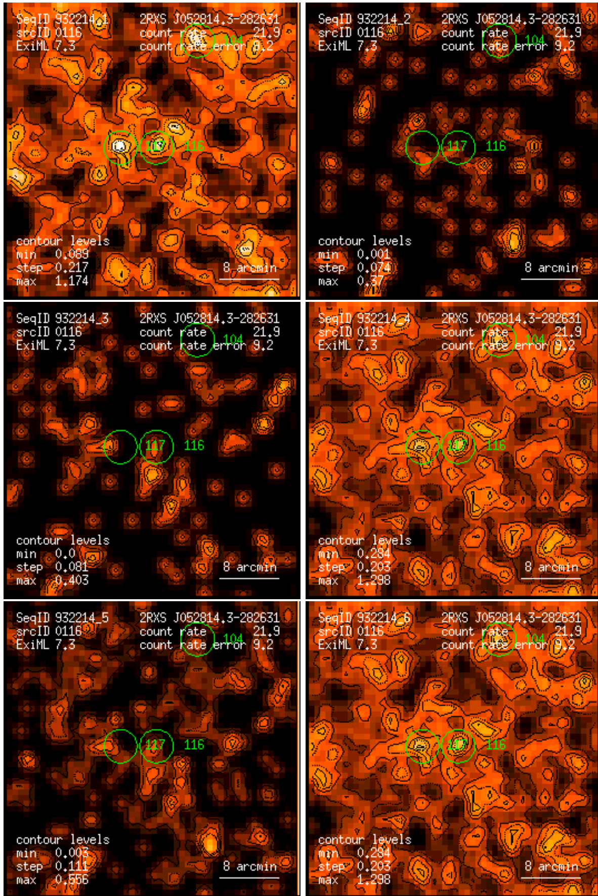
Figure 116: RASS 932214: detection 0116: band rate images, Gaussian filter: (1) PSPC channels 11 – 41, (2) 52 – 90, (3) 91 – 201, (4) 11 – 235, (5) 52 – 201, (6) 11 – 201. Broad band rates in counts/ks. Band rate contour levels in counts/ks/arcmin 2 .
