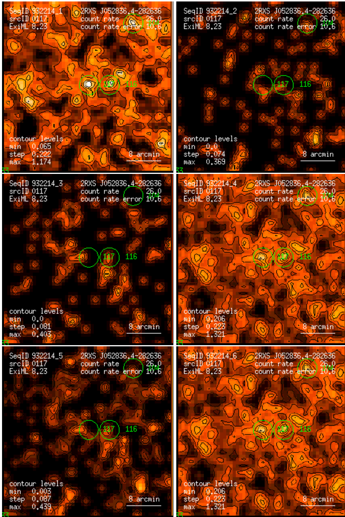
Figure 117: RASS 932214: detection 0117: band rate images, Gaussian filter: (1) PSPC channels 11 – 41, (2) 52 – 90, (3) 91 – 201, (4) 11 – 235, (5) 52 – 201, (6) 11 – 201. Broad band rates in counts/ks. Band rate contour levels in counts/ks/arcmin 2 .
