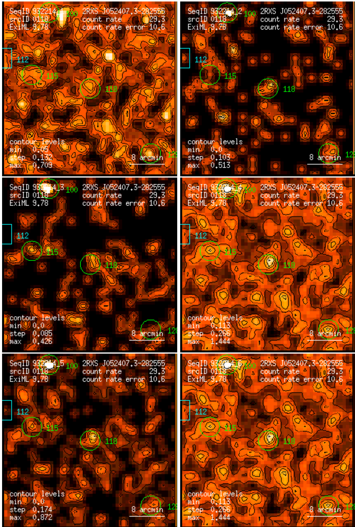
Figure 118: RASS 932214: detection 0118: band rate images, Gaussian filter: (1) PSPC channels 11 – 41, (2) 52 – 90, (3) 91 – 201, (4) 11 – 235, (5) 52 – 201, (6) 11 – 201. Broad band rates in counts/ks. Band rate contour levels in counts/ks/arcmin 2 .
