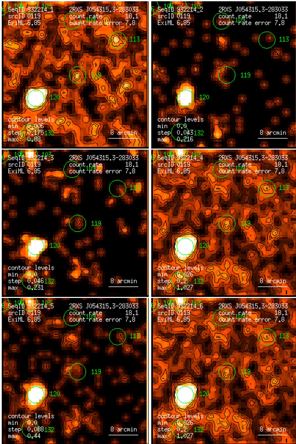
Figure 119: RASS 932214: detection 0119: band rate images, Gaussian filter: (1) PSPC channels 11 – 41, (2) 52 – 90, (3) 91 – 201, (4) 11 – 235, (5) 52 – 201, (6) 11 – 201. Broad band rates in counts/ks. Band rate contour levels in counts/ks/arcmin 2 .
