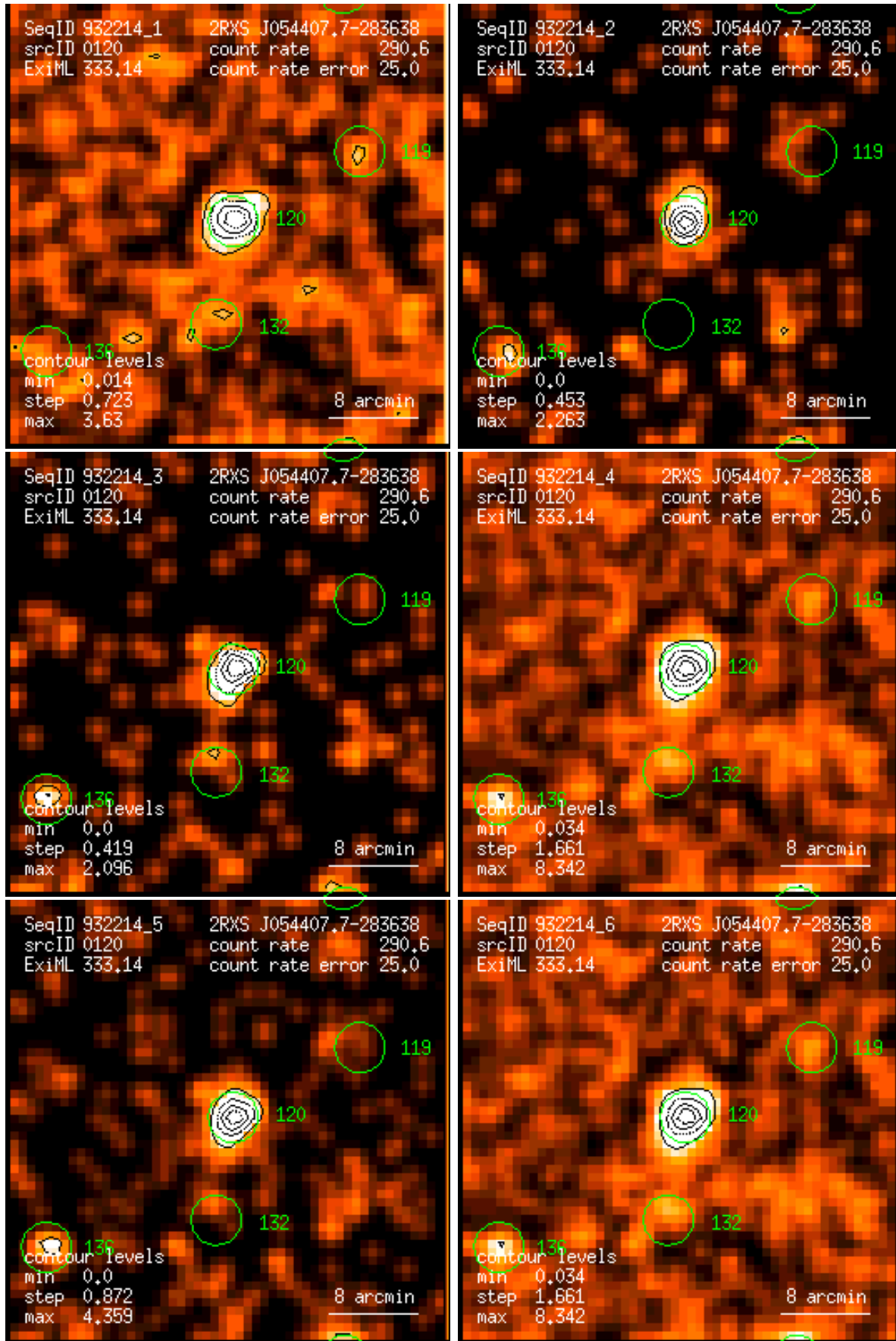
Figure 120: RASS 932214: detection 0120: band rate images, Gaussian filter: (1) PSPC channels 11 – 41, (2) 52 – 90, (3) 91 – 201, (4) 11 – 235, (5) 52 – 201, (6) 11 – 201. Broad band rates in counts/ks. Band rate contour levels in counts/ks/arcmin 2 .
