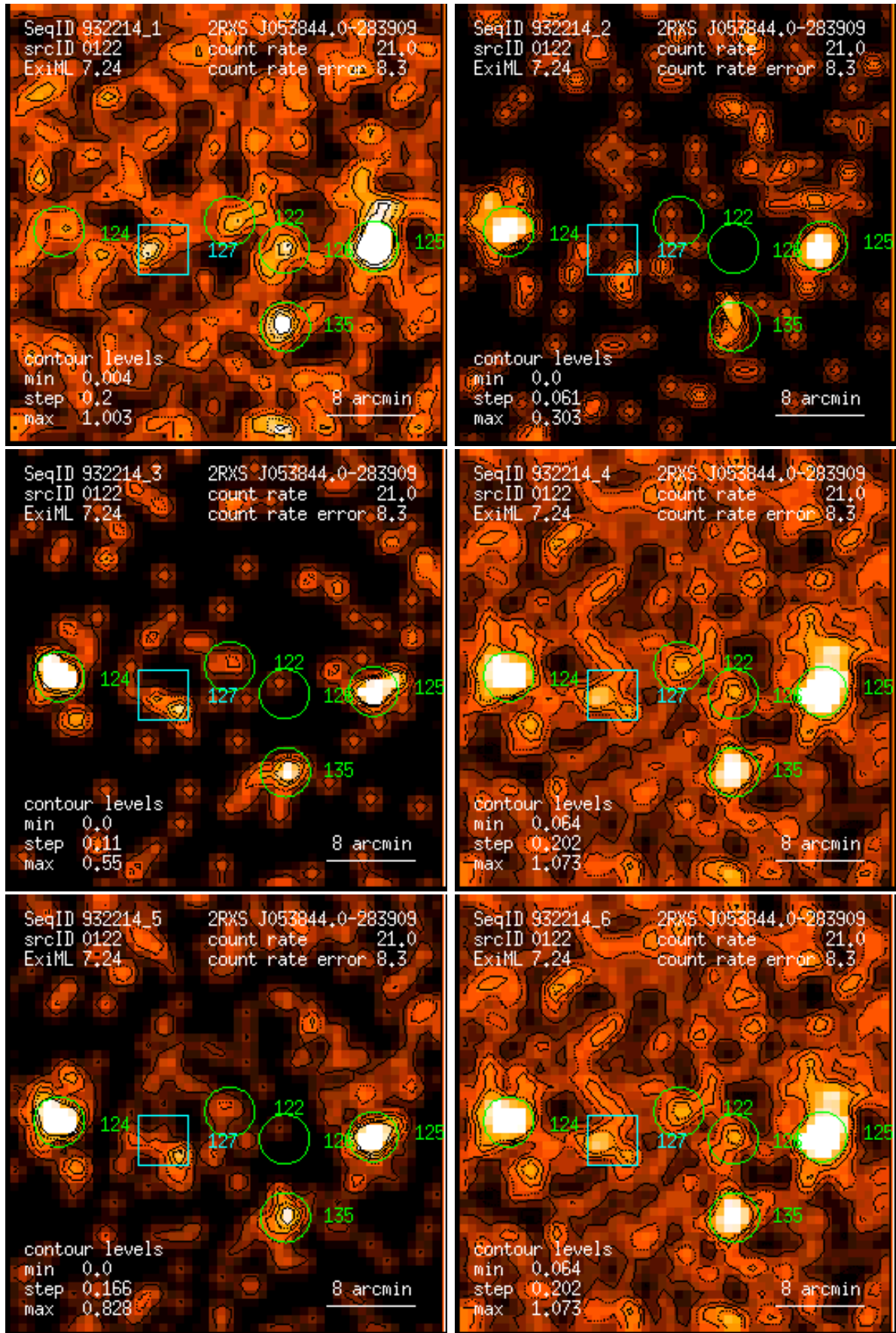
Figure 122: RASS 932214: detection 0122: band rate images, Gaussian filter: (1) PSPC channels 11 – 41, (2) 52 – 90, (3) 91 – 201, (4) 11 – 235, (5) 52 – 201, (6) 11 – 201. Broad band rates in counts/ks. Band rate contour levels in counts/ks/arcmin 2 .
