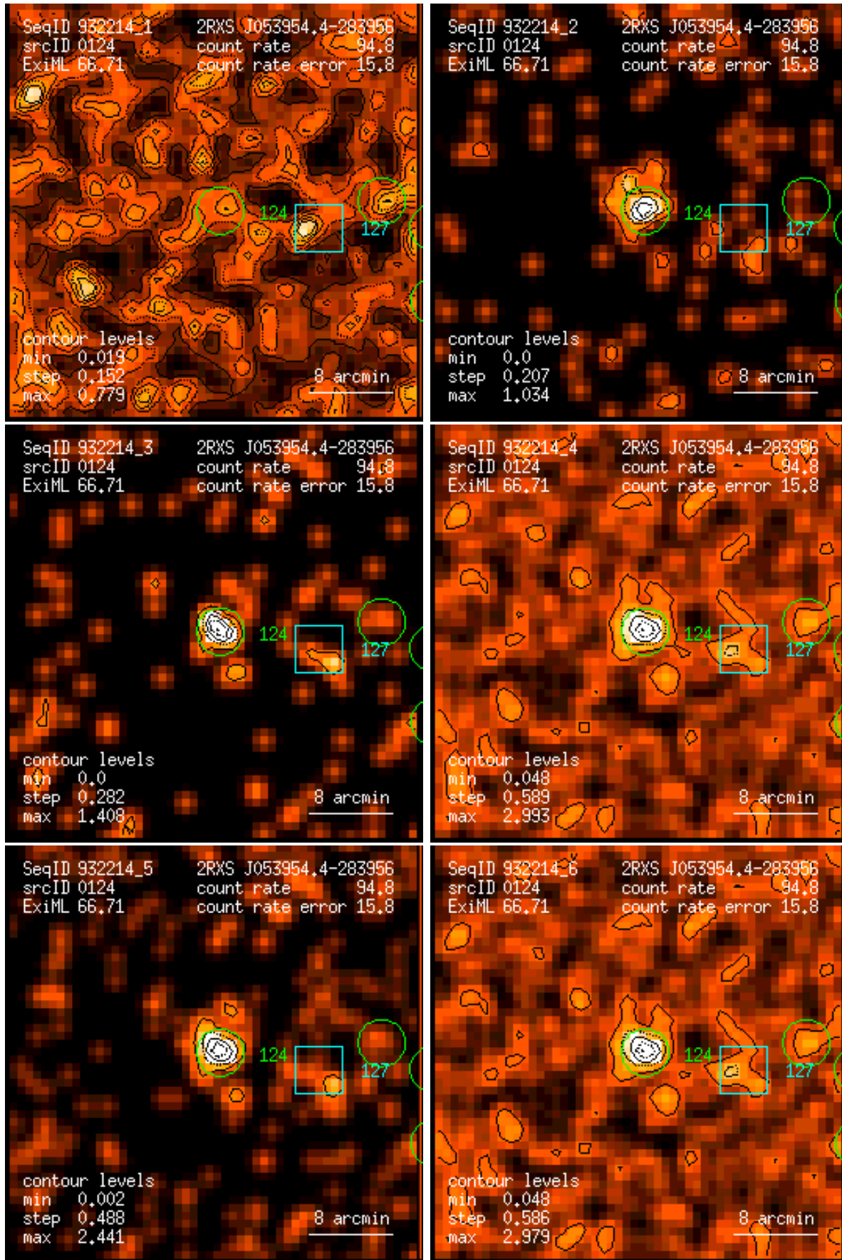
Figure 124: RASS 932214: detection 0124: band rate images, Gaussian filter: (1) PSPC channels 11 – 41, (2) 52 – 90, (3) 91 – 201, (4) 11 – 235, (5) 52 – 201, (6) 11 – 201. Broad band rates in counts/ks. Band rate contour levels in counts/ks/arcmin 2 .
