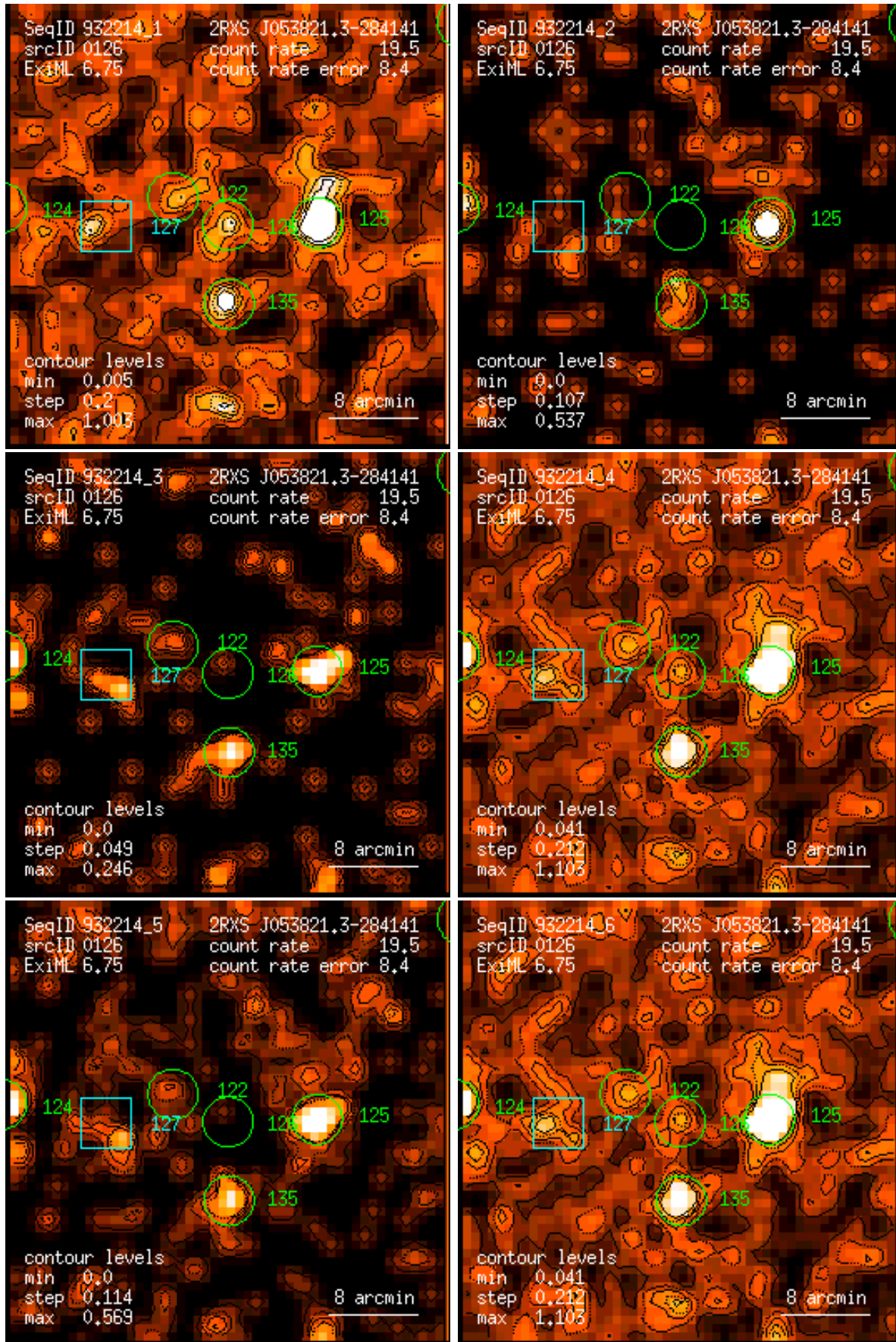
Figure 126: RASS 932214: detection 0126: band rate images, Gaussian filter: (1) PSPC channels 11 – 41, (2) 52 – 90, (3) 91 – 201, (4) 11 – 235, (5) 52 – 201, (6) 11 – 201. Broad band rates in counts/ks. Band rate contour levels in counts/ks/arcmin 2 .
