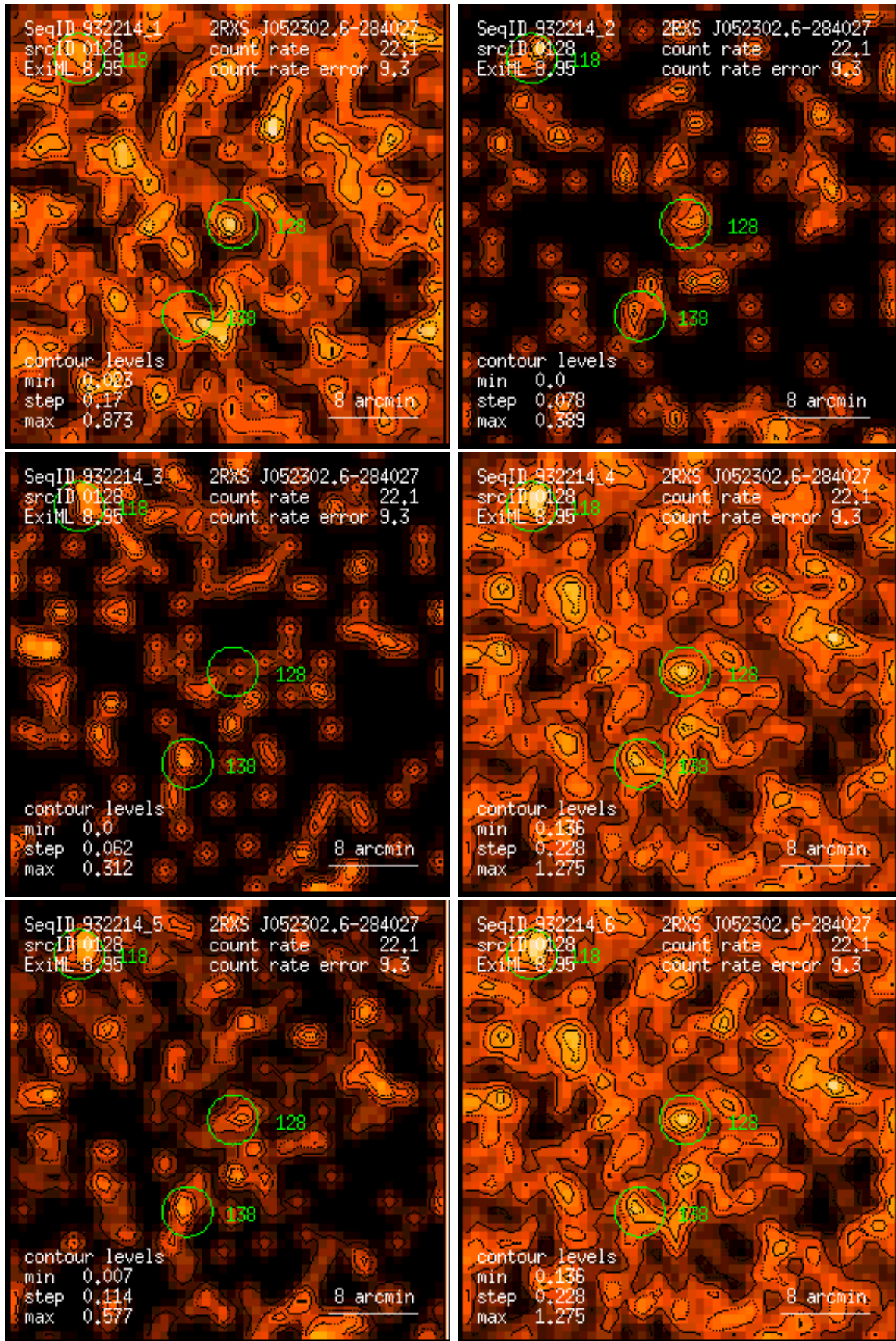
Figure 128: RASS 932214: detection 0128: band rate images, Gaussian filter: (1) PSPC channels 11 – 41, (2) 52 – 90, (3) 91 – 201, (4) 11 – 235, (5) 52 – 201, (6) 11 – 201. Broad band rates in counts/ks. Band rate contour levels in counts/ks/arcmin 2 .
