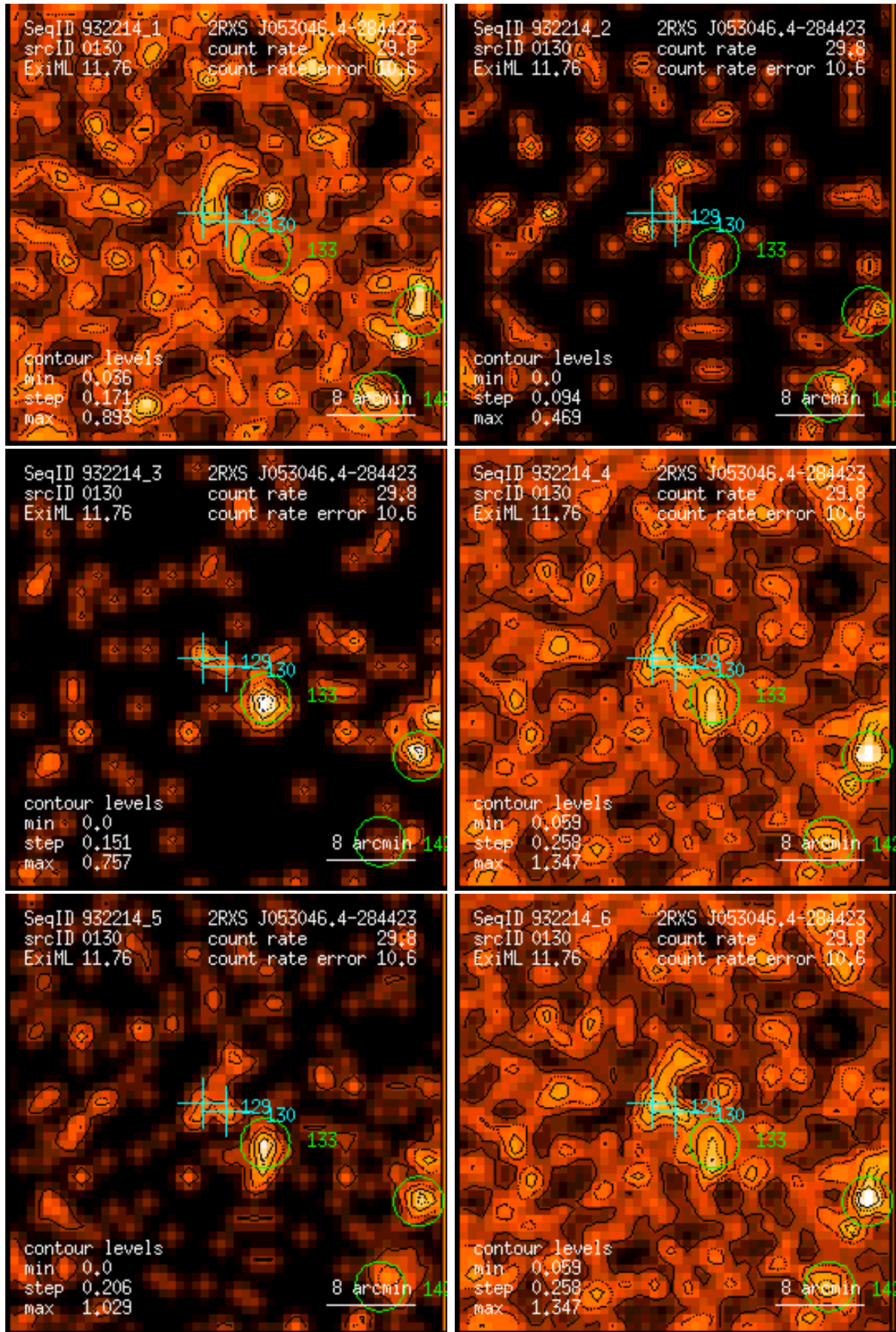
Figure 130: RASS 932214: detection 0130: band rate images, Gaussian filter: (1) PSPC channels 11 – 41, (2) 52 – 90, (3) 91 – 201, (4) 11 – 235, (5) 52 – 201, (6) 11 – 201. Broad band rates in counts/ks. Band rate contour levels in counts/ks/arcmin 2 .
