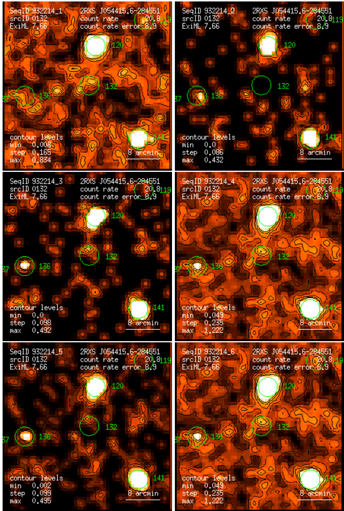
Figure 132: RASS 932214: detection 0132: band rate images, Gaussian filter: (1) PSPC channels 11 – 41, (2) 52 – 90, (3) 91 – 201, (4) 11 – 235, (5) 52 – 201, (6) 11 – 201. Broad band rates in counts/ks. Band rate contour levels in counts/ks/arcmin 2 .
