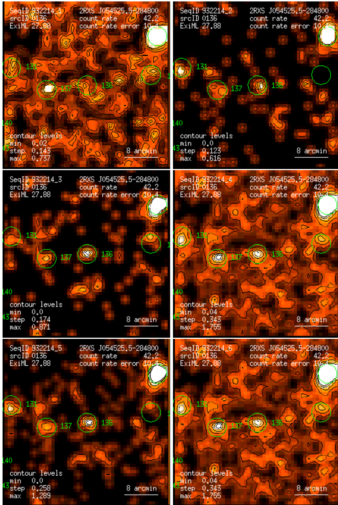
Figure 136: RASS 932214: detection 0136: band rate images, Gaussian filter: (1) PSPC channels 11 – 41, (2) 52 – 90, (3) 91 – 201, (4) 11 – 235, (5) 52 – 201, (6) 11 – 201. Broad band rates in counts/ks. Band rate contour levels in counts/ks/arcmin 2 .
