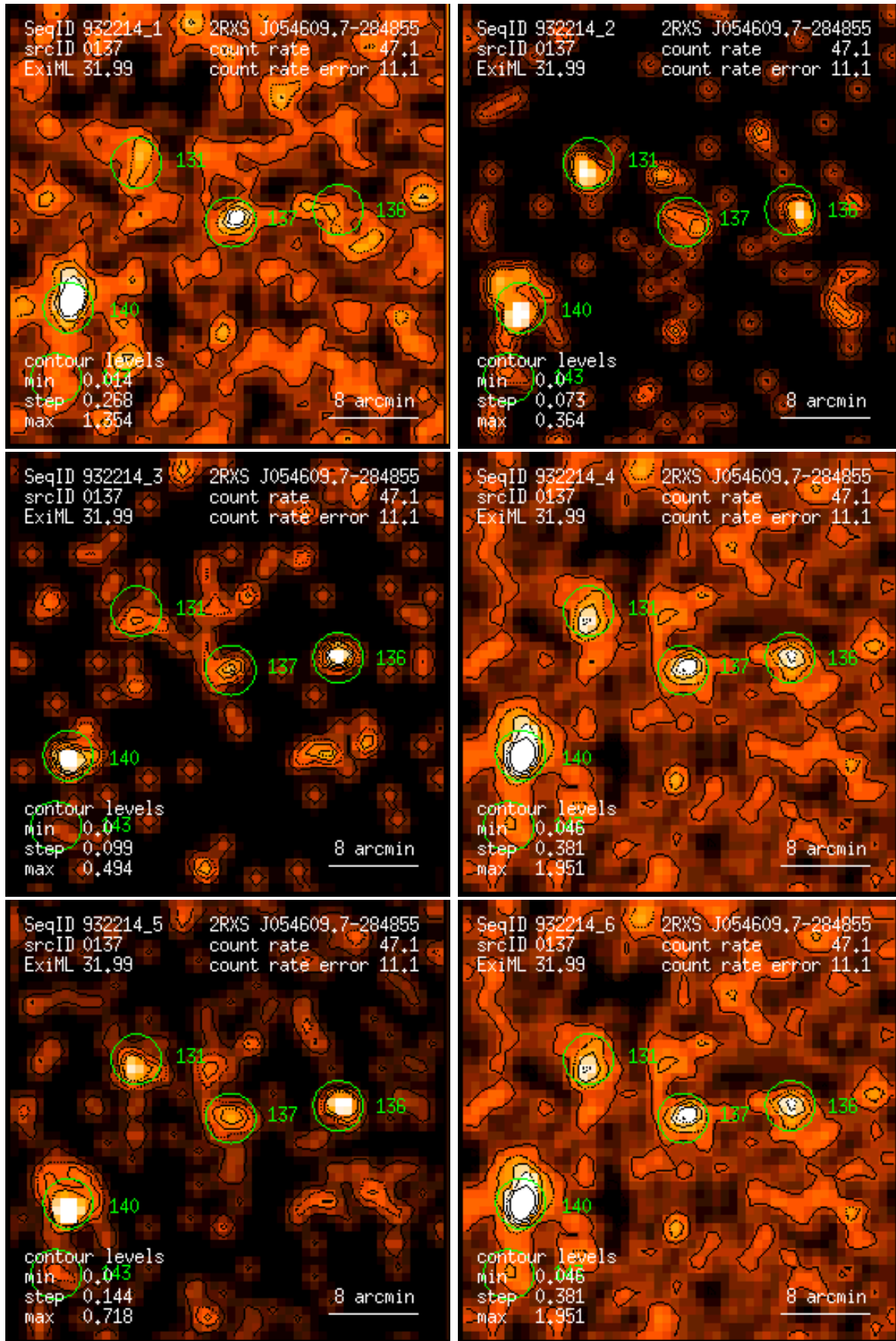
Figure 137: RASS 932214: detection 0137: band rate images, Gaussian filter: (1) PSPC channels 11 – 41, (2) 52 – 90, (3) 91 – 201, (4) 11 – 235, (5) 52 – 201, (6) 11 – 201. Broad band rates in counts/ks. Band rate contour levels in counts/ks/arcmin 2 .
