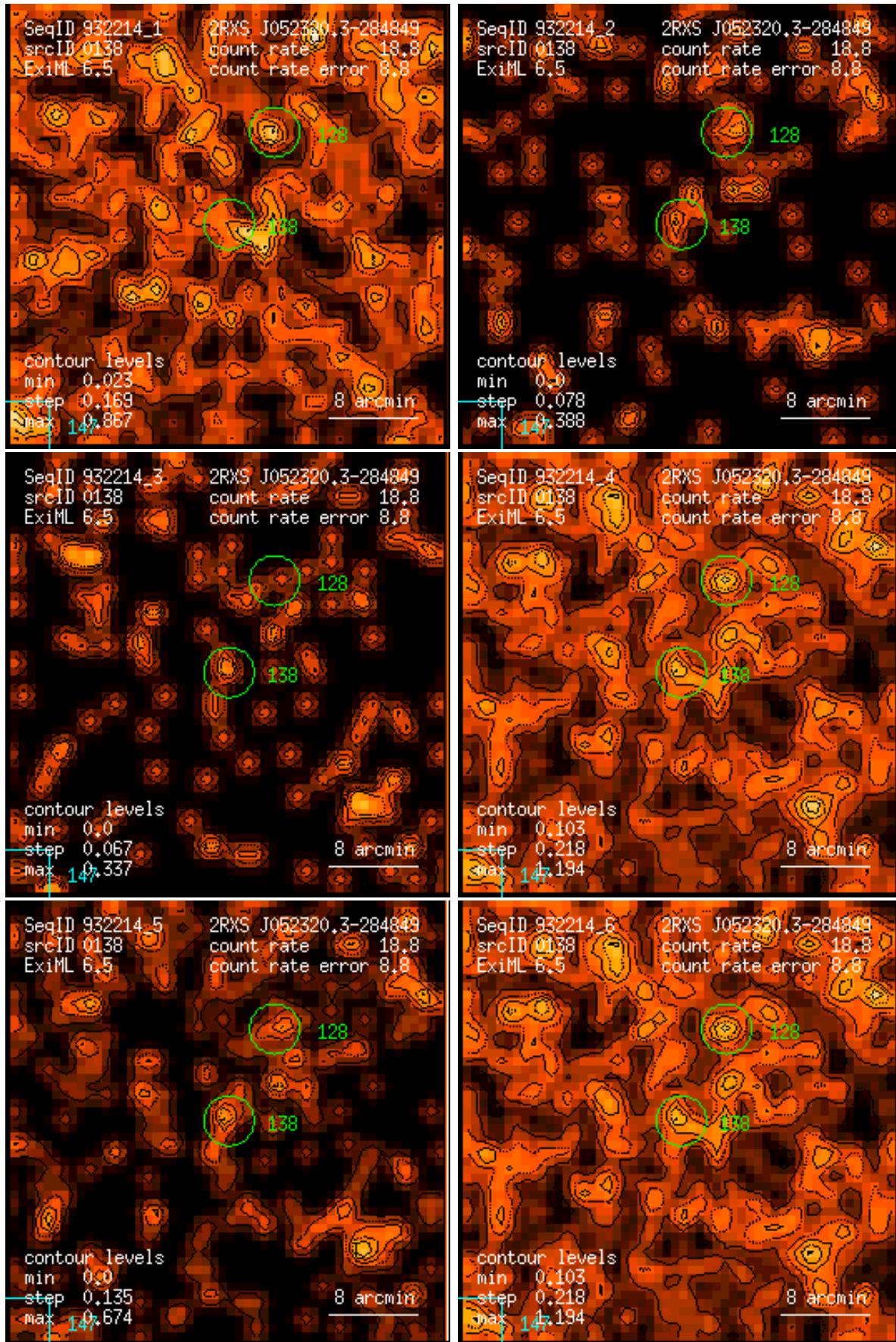
Figure 138: RASS 932214: detection 0138: band rate images, Gaussian filter: (1) PSPC channels 11 – 41, (2) 52 – 90, (3) 91 – 201, (4) 11 – 235, (5) 52 – 201, (6) 11 – 201. Broad band rates in counts/ks. Band rate contour levels in counts/ks/arcmin 2 .
