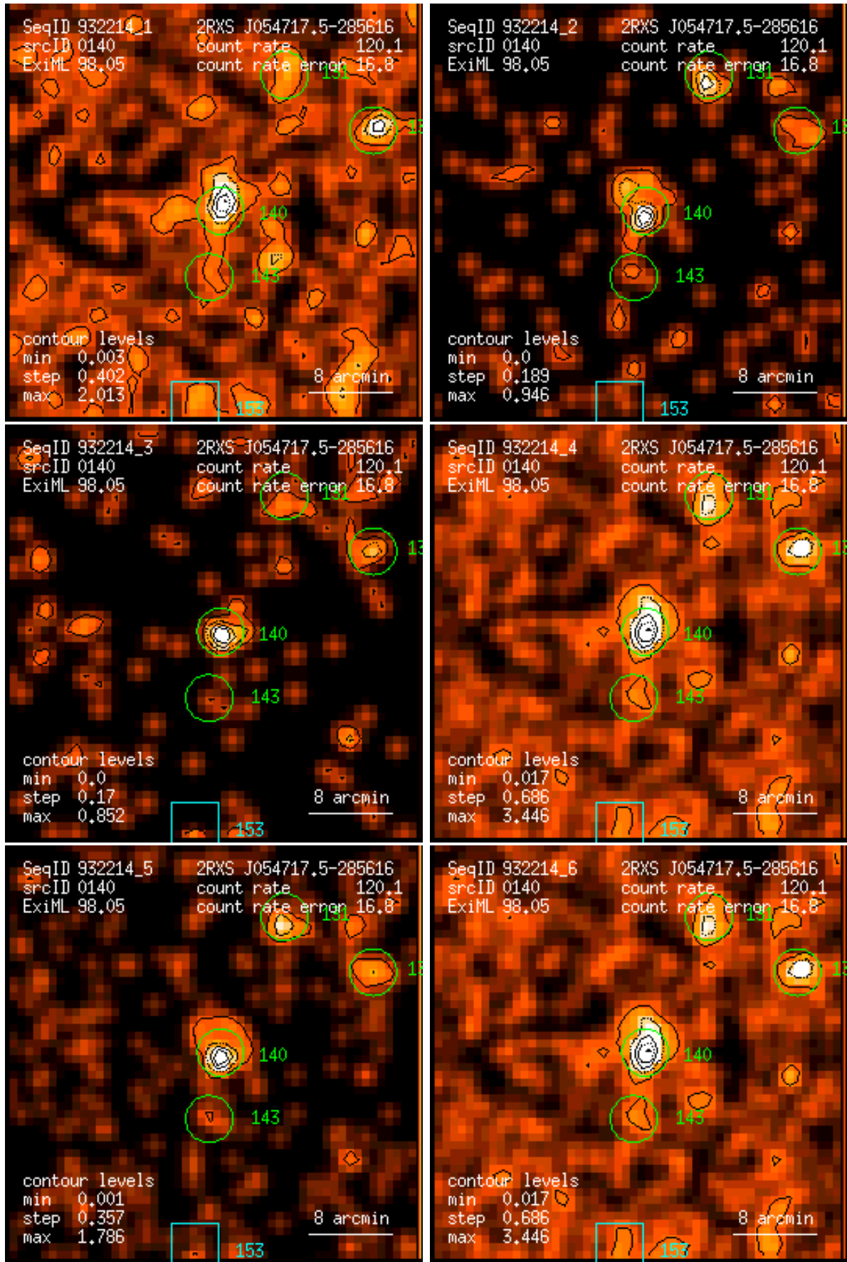
Figure 140: RASS 932214: detection 0140: band rate images, Gaussian filter: (1) PSPC channels 11 – 41, (2) 52 – 90, (3) 91 – 201, (4) 11 – 235, (5) 52 – 201, (6) 11 – 201. Broad band rates in counts/ks. Band rate contour levels in counts/ks/arcmin 2 .
