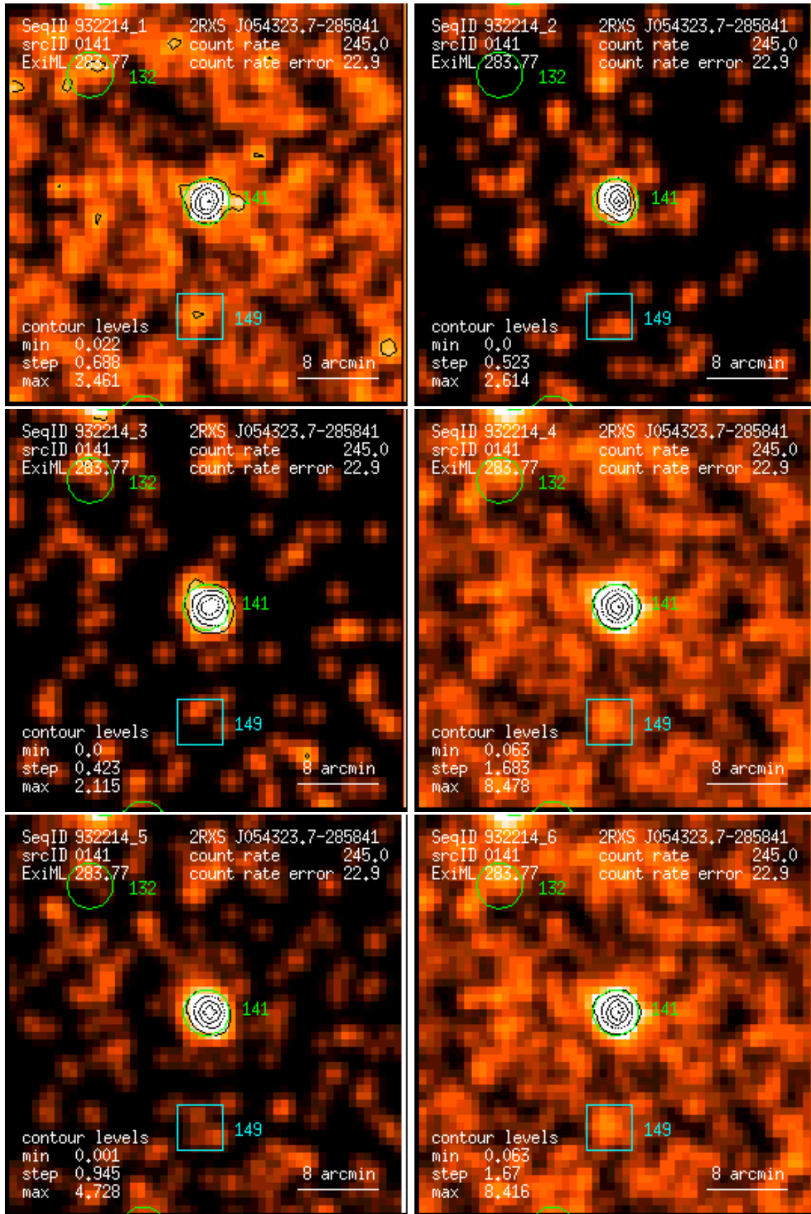
Figure 141: RASS 932214: detection 0141: band rate images, Gaussian filter: (1) PSPC channels 11 – 41, (2) 52 – 90, (3) 91 – 201, (4) 11 – 235, (5) 52 – 201, (6) 11 – 201. Broad band rates in counts/ks. Band rate contour levels in counts/ks/arcmin 2 .
