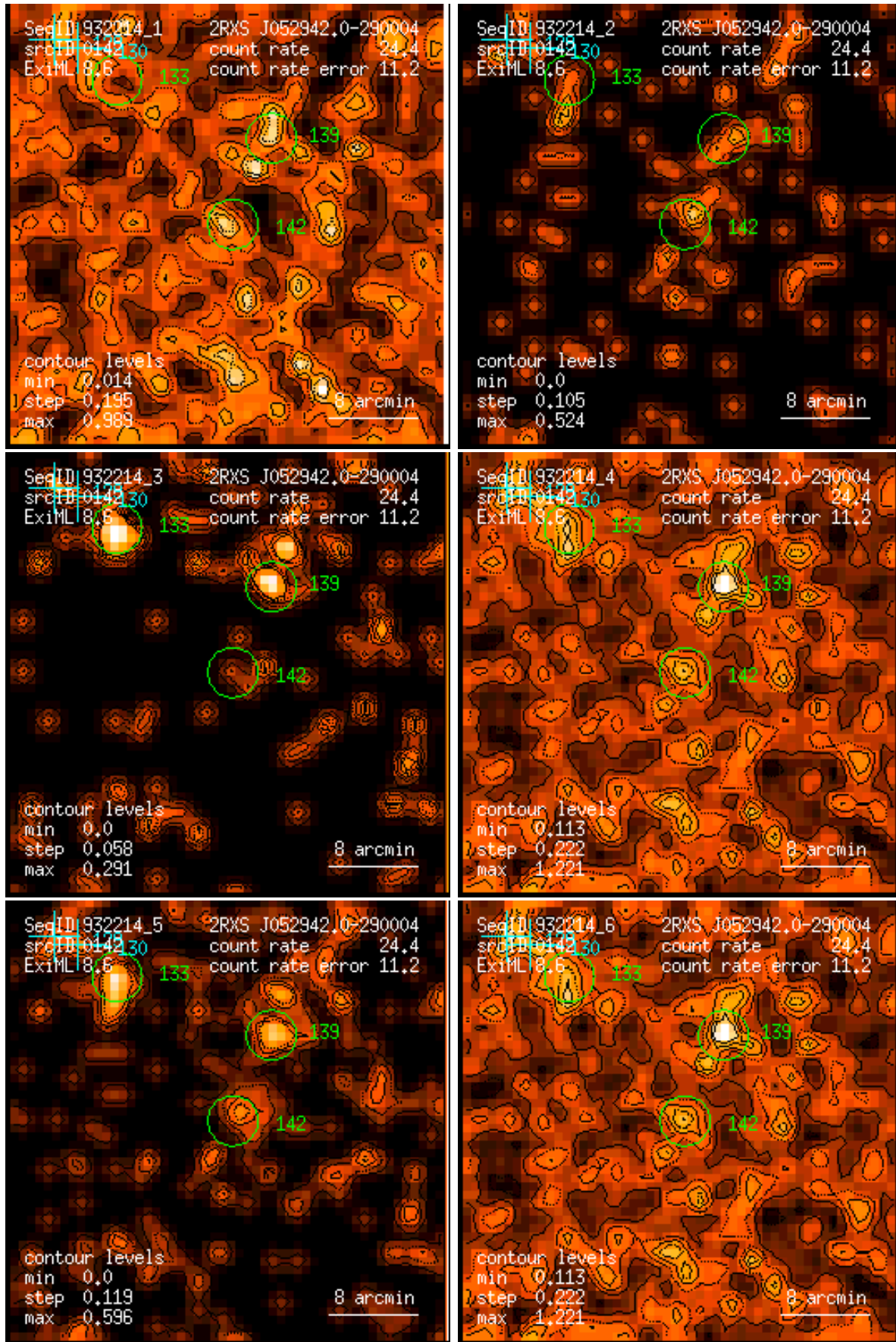
Figure 142: RASS 932214: detection 0142: band rate images, Gaussian filter: (1) PSPC channels 11 – 41, (2) 52 – 90, (3) 91 – 201, (4) 11 – 235, (5) 52 – 201, (6) 11 – 201. Broad band rates in counts/ks. Band rate contour levels in counts/ks/arcmin 2 .
