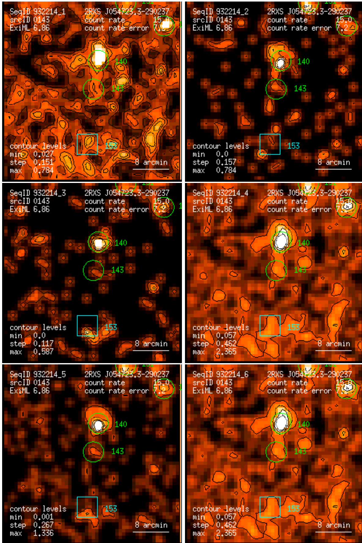
Figure 143: RASS 932214: detection 0143: band rate images, Gaussian filter: (1) PSPC channels 11 – 41, (2) 52 – 90, (3) 91 – 201, (4) 11 – 235, (5) 52 – 201, (6) 11 – 201. Broad band rates in counts/ks. Band rate contour levels in counts/ks/arcmin 2 .
