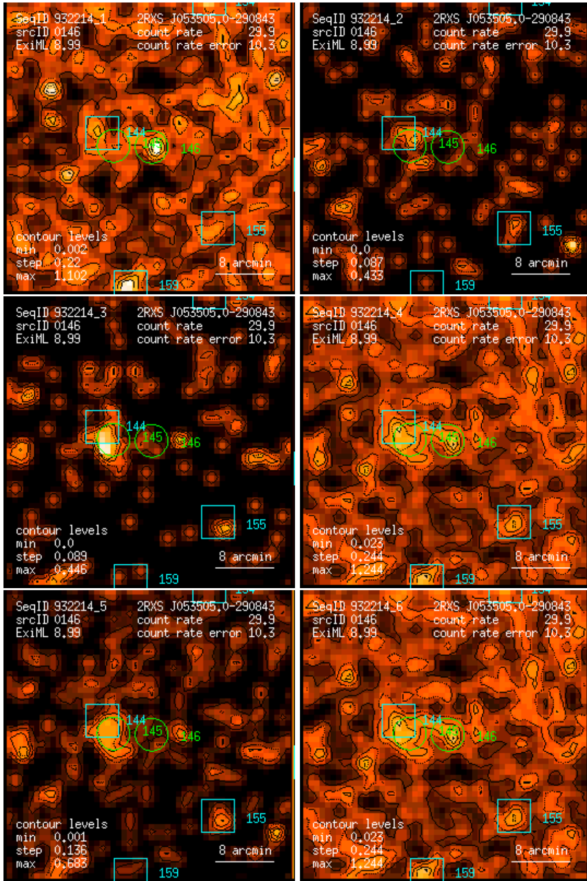
Figure 146: RASS 932214: detection 0146: band rate images, Gaussian filter: (1) PSPC channels 11 – 41, (2) 52 – 90, (3) 91 – 201, (4) 11 – 235, (5) 52 – 201, (6) 11 – 201. Broad band rates in counts/ks. Band rate contour levels in counts/ks/arcmin 2 .
