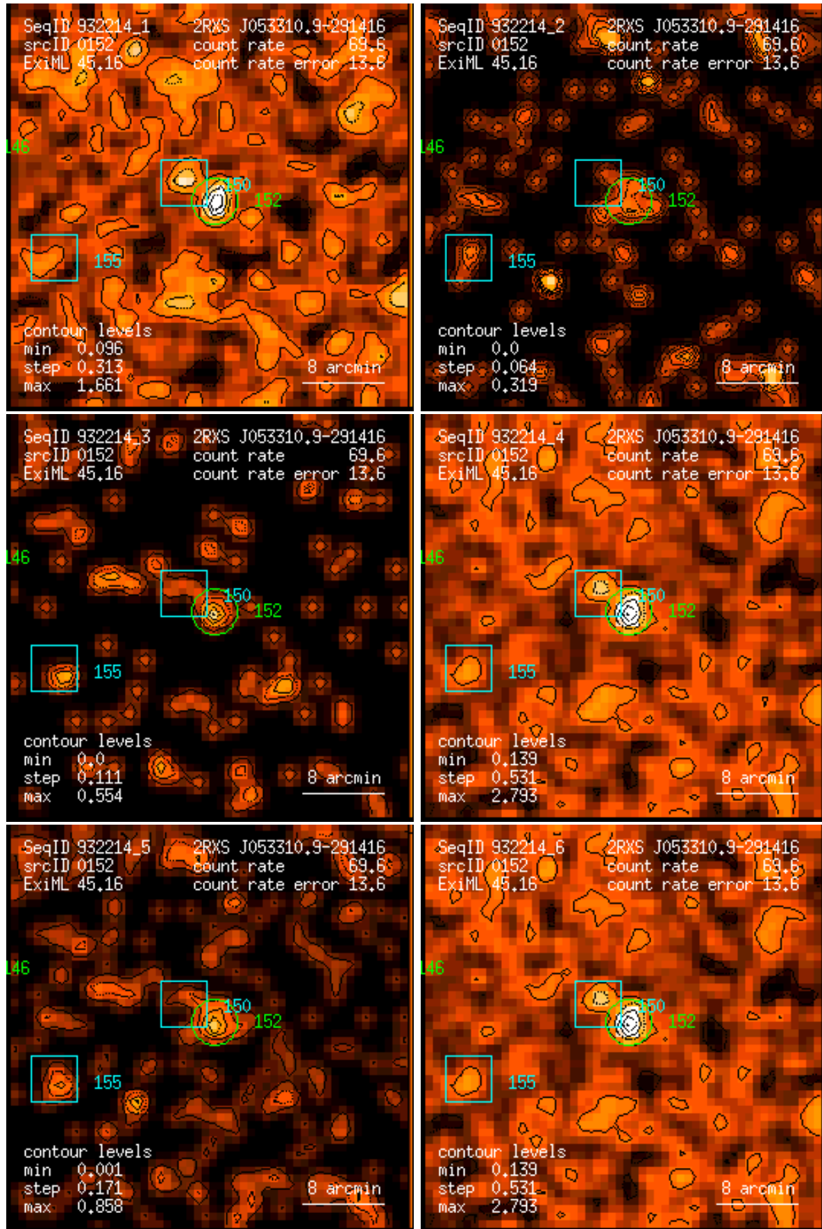
Figure 152: RASS 932214: detection 0152: band rate images, Gaussian filter: (1) PSPC channels 11 – 41, (2) 52 – 90, (3) 91 – 201, (4) 11 – 235, (5) 52 – 201, (6) 11 – 201. Broad band rates in counts/ks. Band rate contour levels in counts/ks/arcmin 2 .
