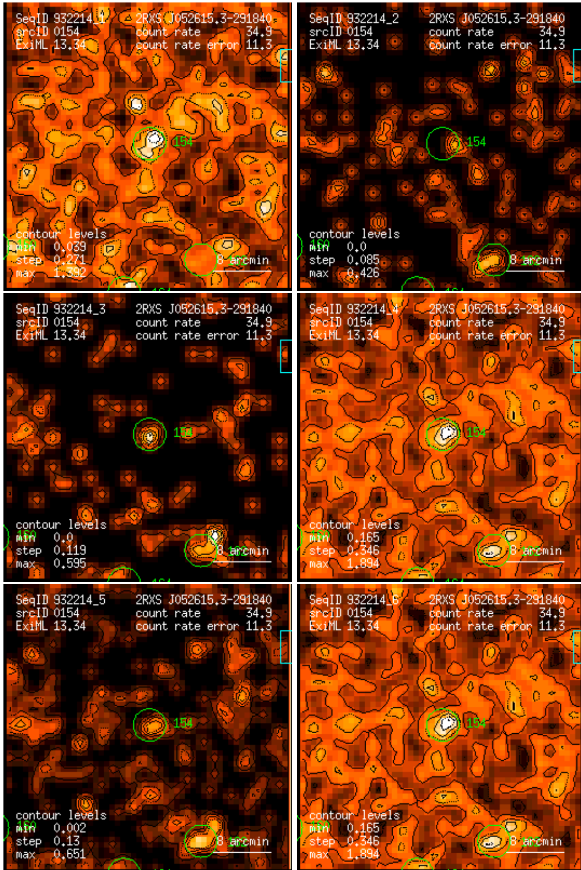
Figure 154: RASS 932214: detection 0154: band rate images, Gaussian filter: (1) PSPC channels 11 – 41, (2) 52 – 90, (3) 91 – 201, (4) 11 – 235, (5) 52 – 201, (6) 11 – 201. Broad band rates in counts/ks. Band rate contour levels in counts/ks/arcmin 2 .
