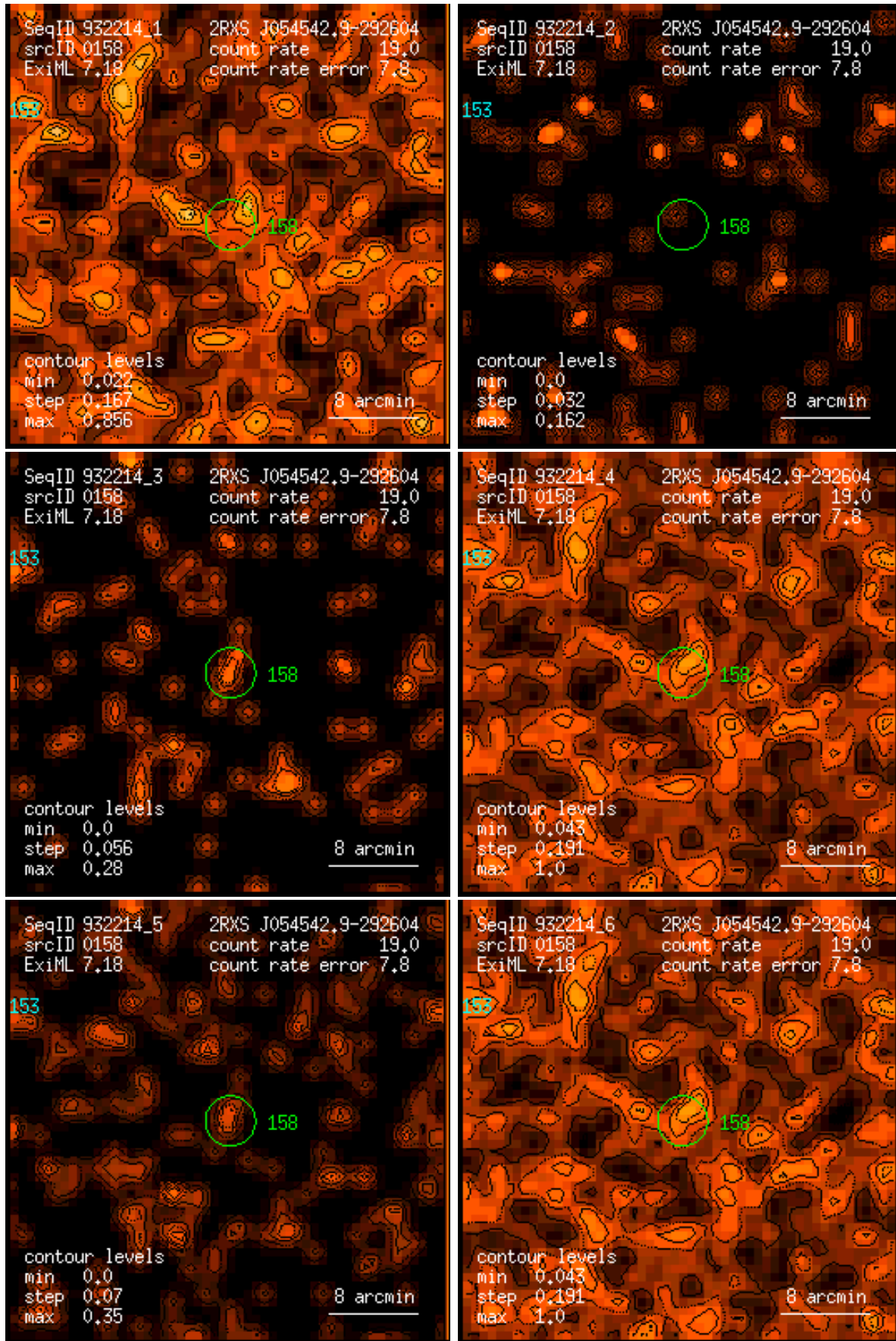
Figure 158: RASS 932214: detection 0158: band rate images, Gaussian filter: (1) PSPC channels 11 – 41, (2) 52 – 90, (3) 91 – 201, (4) 11 – 235, (5) 52 – 201, (6) 11 – 201. Broad band rates in counts/ks. Band rate contour levels in counts/ks/arcmin 2 .
