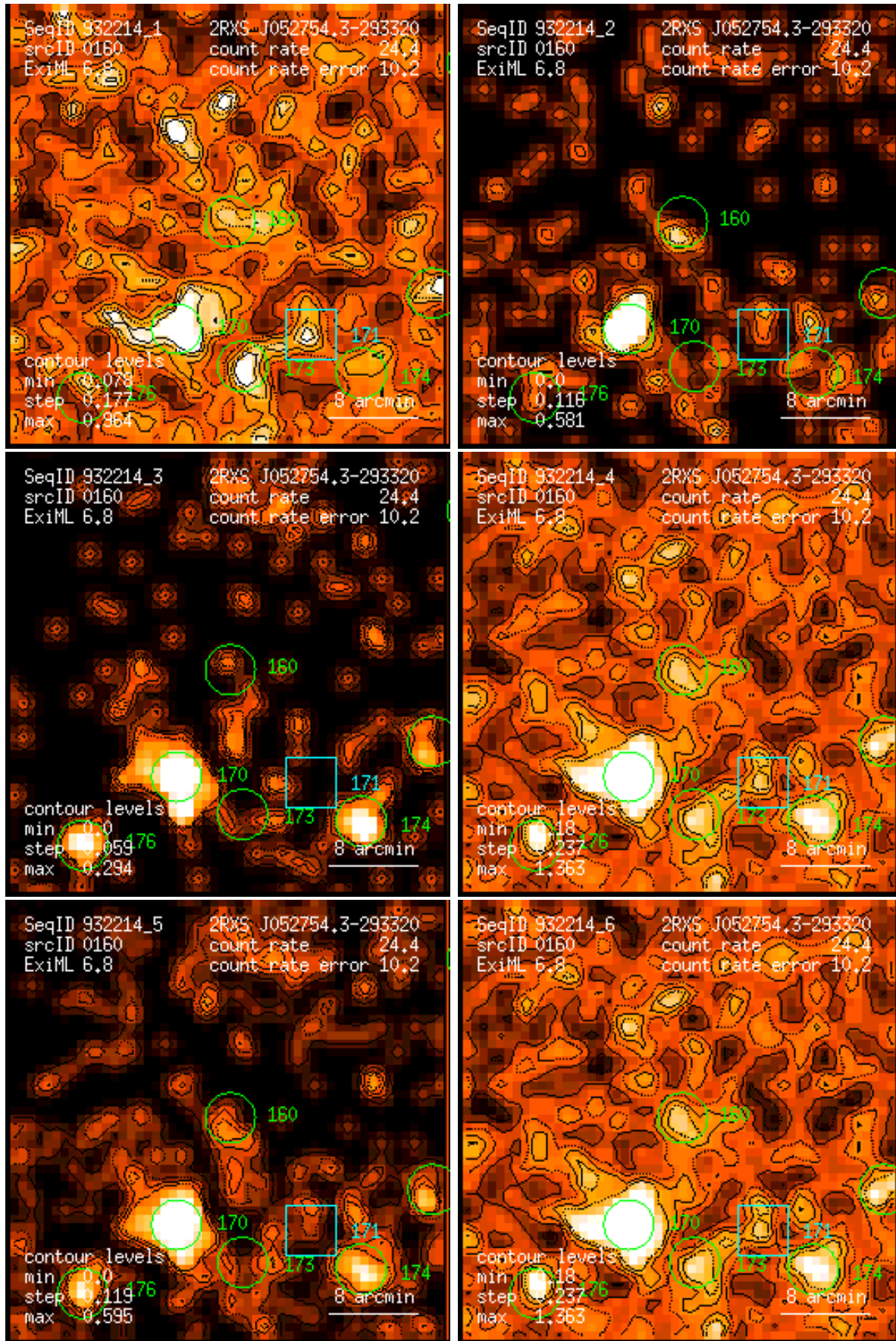
Figure 160: RASS 932214: detection 0160: band rate images, Gaussian filter: (1) PSPC channels 11 – 41, (2) 52 – 90, (3) 91 – 201, (4) 11 – 235, (5) 52 – 201, (6) 11 – 201. Broad band rates in counts/ks. Band rate contour levels in counts/ks/arcmin 2 .
