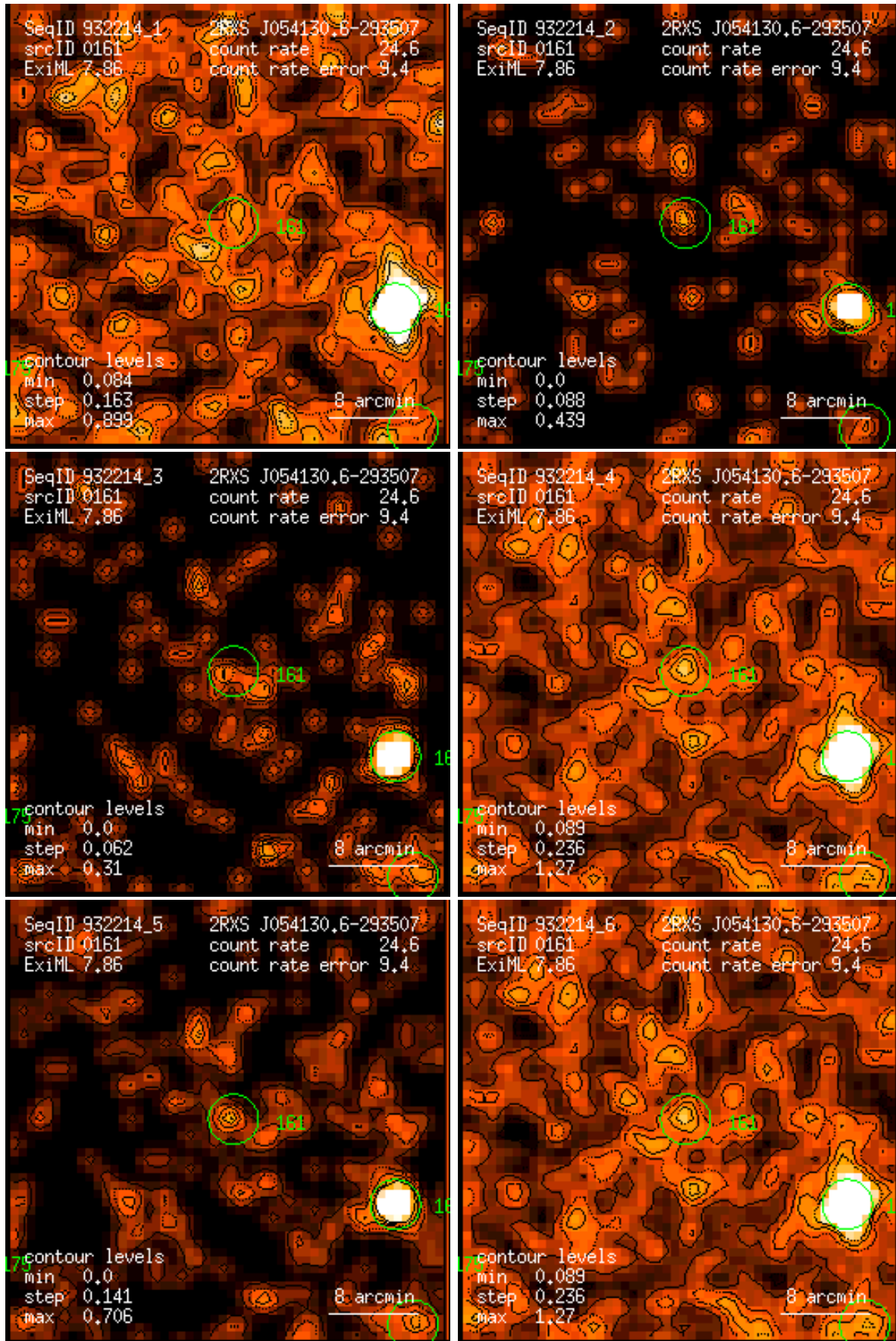
Figure 161: RASS 932214: detection 0161: band rate images, Gaussian filter: (1) PSPC channels 11 – 41, (2) 52 – 90, (3) 91 – 201, (4) 11 – 235, (5) 52 – 201, (6) 11 – 201. Broad band rates in counts/ks. Band rate contour levels in counts/ks/arcmin 2 .
