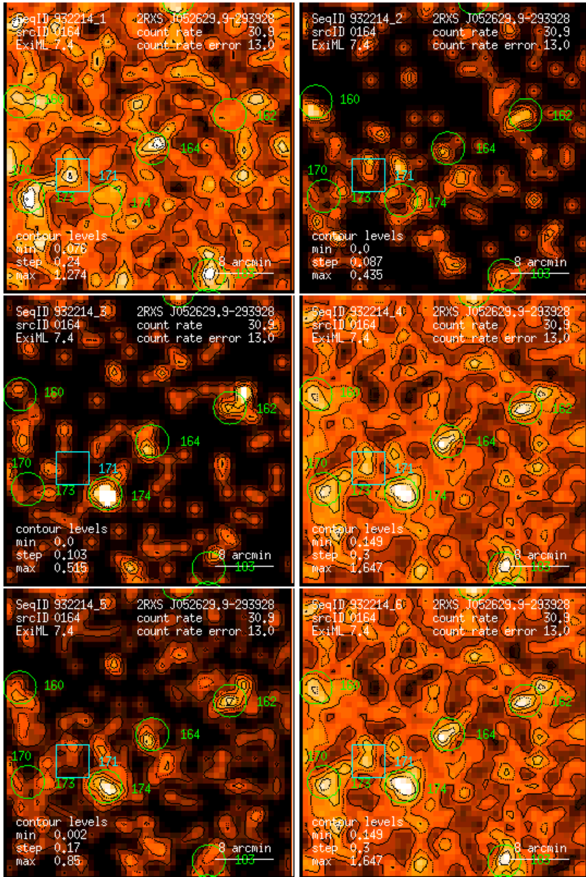
Figure 164: RASS 932214: detection 0164: band rate images, Gaussian filter: (1) PSPC channels 11 – 41, (2) 52 – 90, (3) 91 – 201, (4) 11 – 235, (5) 52 – 201, (6) 11 – 201. Broad band rates in counts/ks. Band rate contour levels in counts/ks/arcmin 2 .
