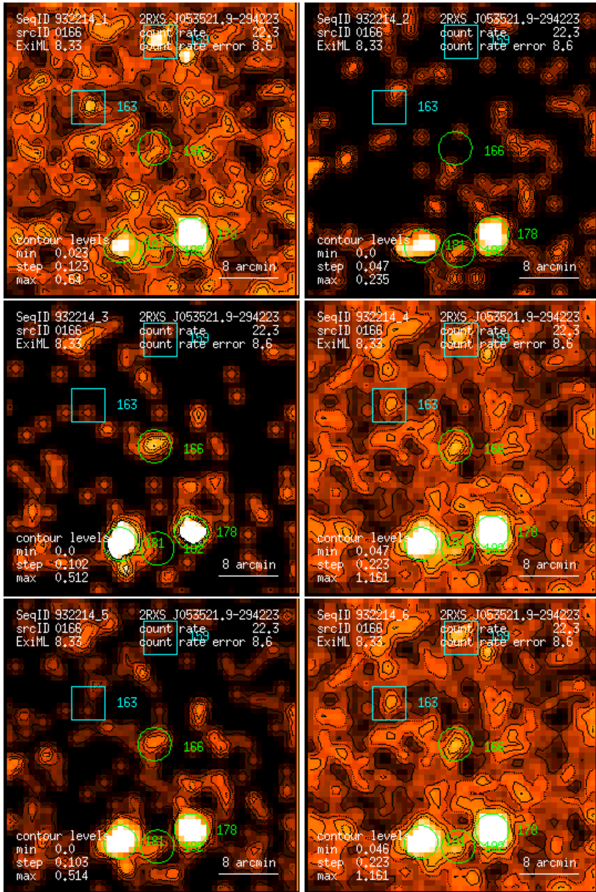
Figure 166: RASS 932214: detection 0166: band rate images, Gaussian filter: (1) PSPC channels 11 – 41, (2) 52 – 90, (3) 91 – 201, (4) 11 – 235, (5) 52 – 201, (6) 11 – 201. Broad band rates in counts/ks. Band rate contour levels in counts/ks/arcmin 2 .
