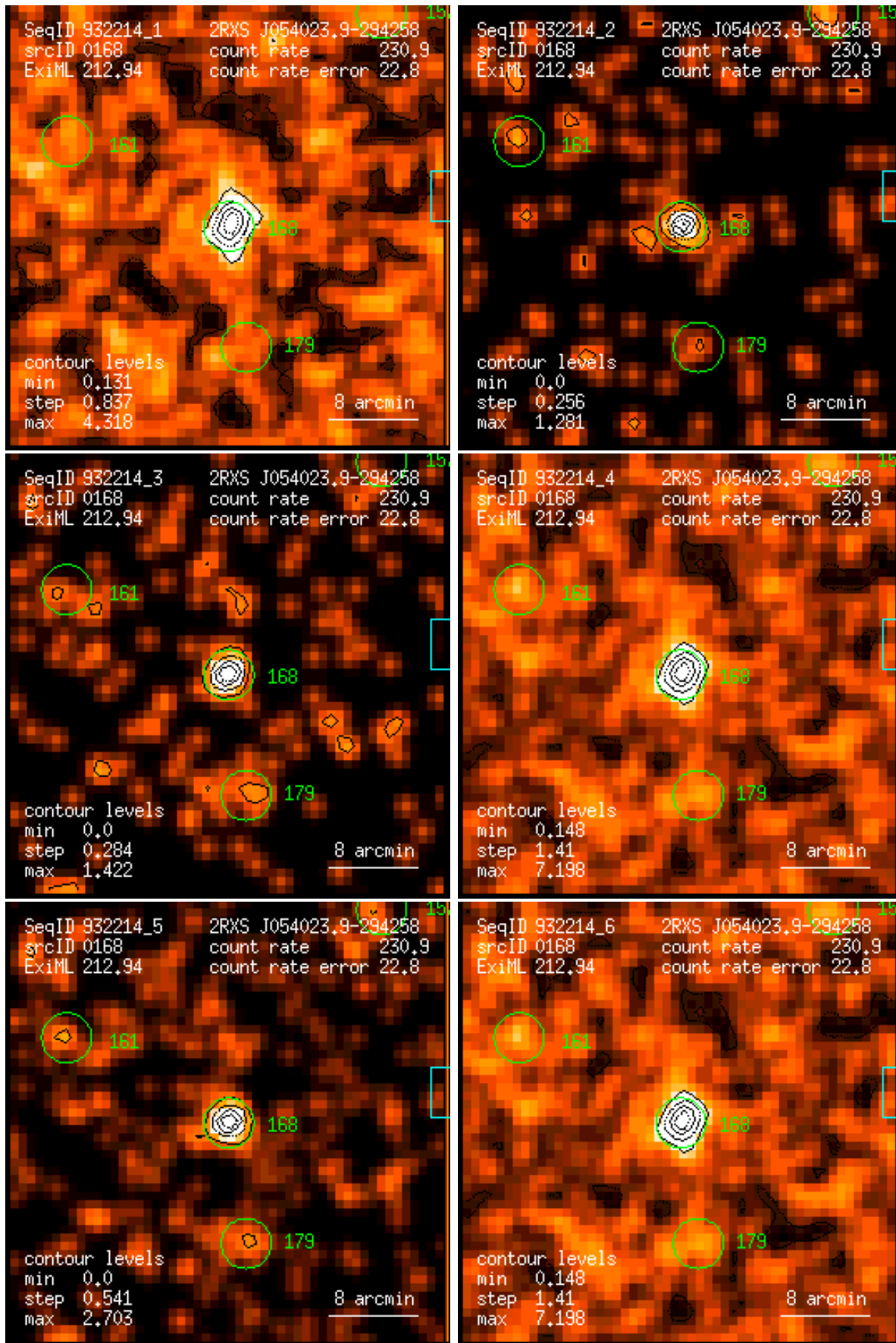
Figure 168: RASS 932214: detection 0168: band rate images, Gaussian filter: (1) PSPC channels 11 – 41, (2) 52 – 90, (3) 91 – 201, (4) 11 – 235, (5) 52 – 201, (6) 11 – 201. Broad band rates in counts/ks. Band rate contour levels in counts/ks/arcmin 2 .
