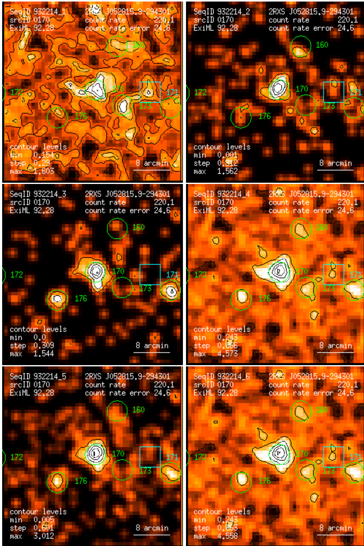
Figure 170: RASS 932214: detection 0170: band rate images, Gaussian filter: (1) PSPC channels 11 – 41, (2) 52 – 90, (3) 91 – 201, (4) 11 – 235, (5) 52 – 201, (6) 11 – 201. Broad band rates in counts/ks. Band rate contour levels in counts/ks/arcmin 2 .
