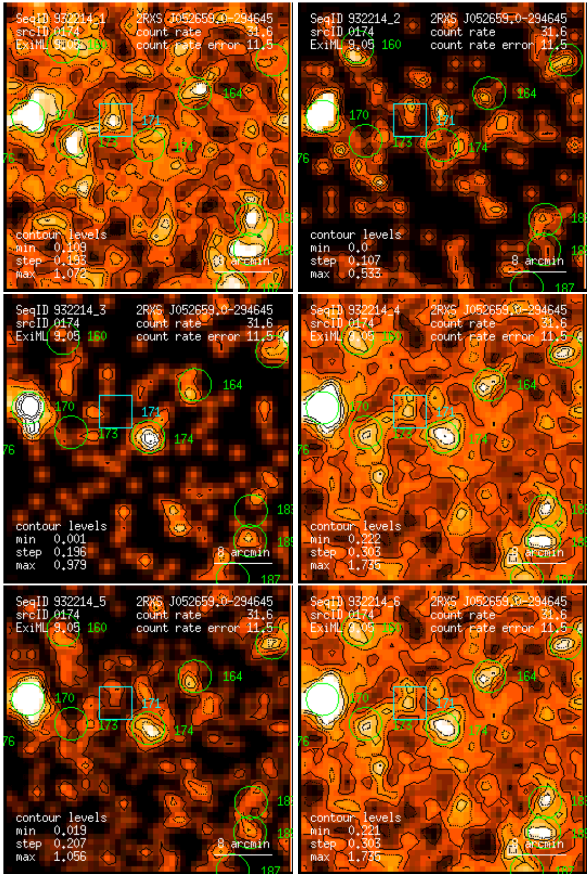
Figure 174: RASS 932214: detection 0174: band rate images, Gaussian filter: (1) PSPC channels 11 – 41, (2) 52 – 90, (3) 91 – 201, (4) 11 – 235, (5) 52 – 201, (6) 11 – 201. Broad band rates in counts/ks. Band rate contour levels in counts/ks/arcmin 2 .
