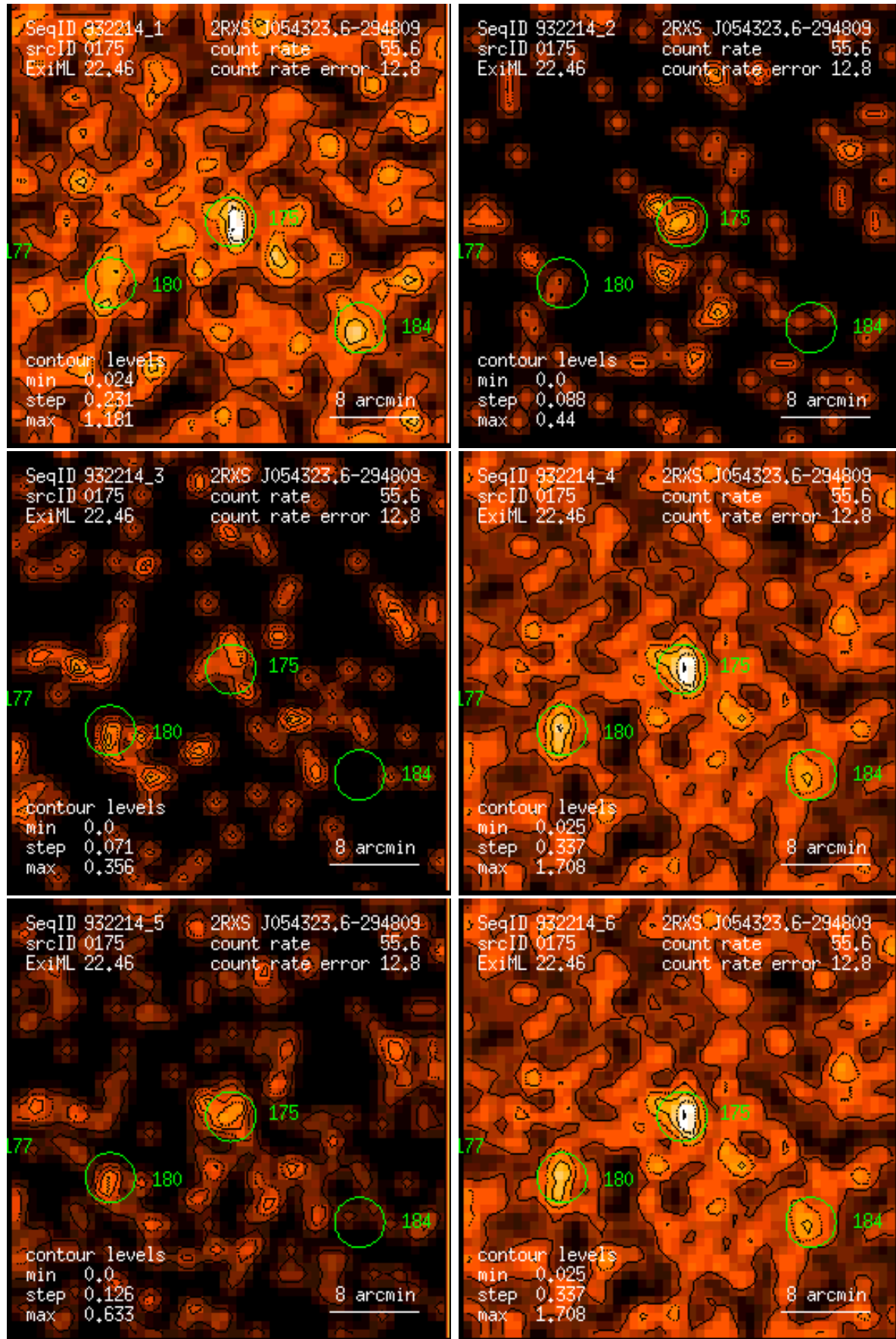
Figure 175: RASS 932214: detection 0175: band rate images, Gaussian filter: (1) PSPC channels 11 – 41, (2) 52 – 90, (3) 91 – 201, (4) 11 – 235, (5) 52 – 201, (6) 11 – 201. Broad band rates in counts/ks. Band rate contour levels in counts/ks/arcmin 2 .
