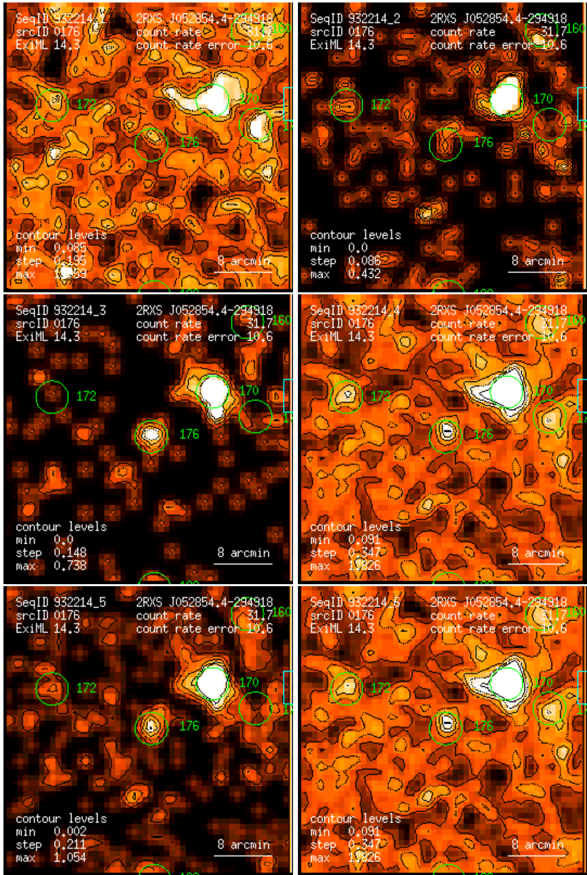
Figure 176: RASS 932214: detection 0176: band rate images, Gaussian filter: (1) PSPC channels 11 – 41, (2) 52 – 90, (3) 91 – 201, (4) 11 – 235, (5) 52 – 201, (6) 11 – 201. Broad band rates in counts/ks. Band rate contour levels in counts/ks/arcmin 2 .
