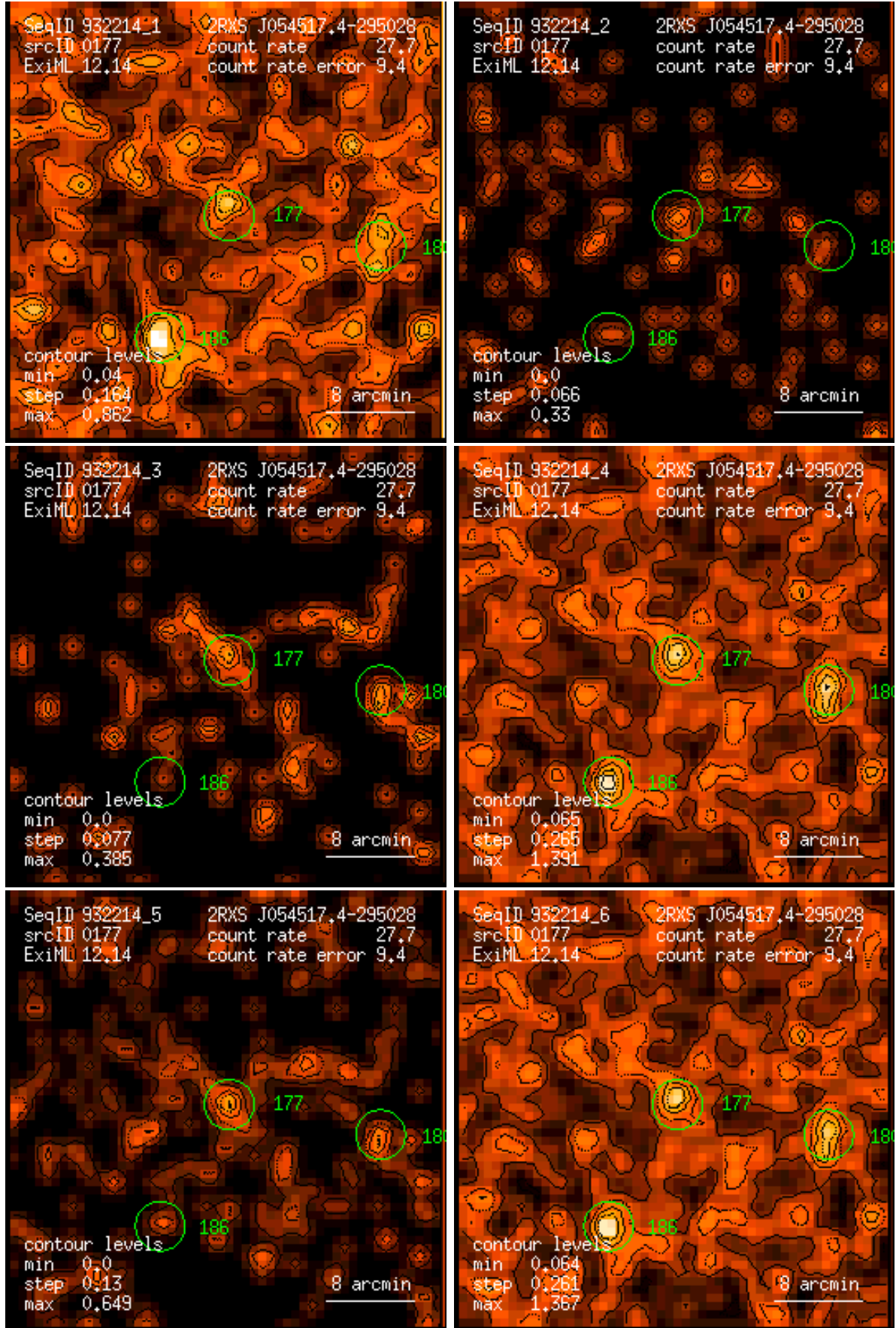
Figure 177: RASS 932214: detection 0177: band rate images, Gaussian filter: (1) PSPC channels 11 – 41, (2) 52 – 90, (3) 91 – 201, (4) 11 – 235, (5) 52 – 201, (6) 11 – 201. Broad band rates in counts/ks. Band rate contour levels in counts/ks/arcmin 2 .
