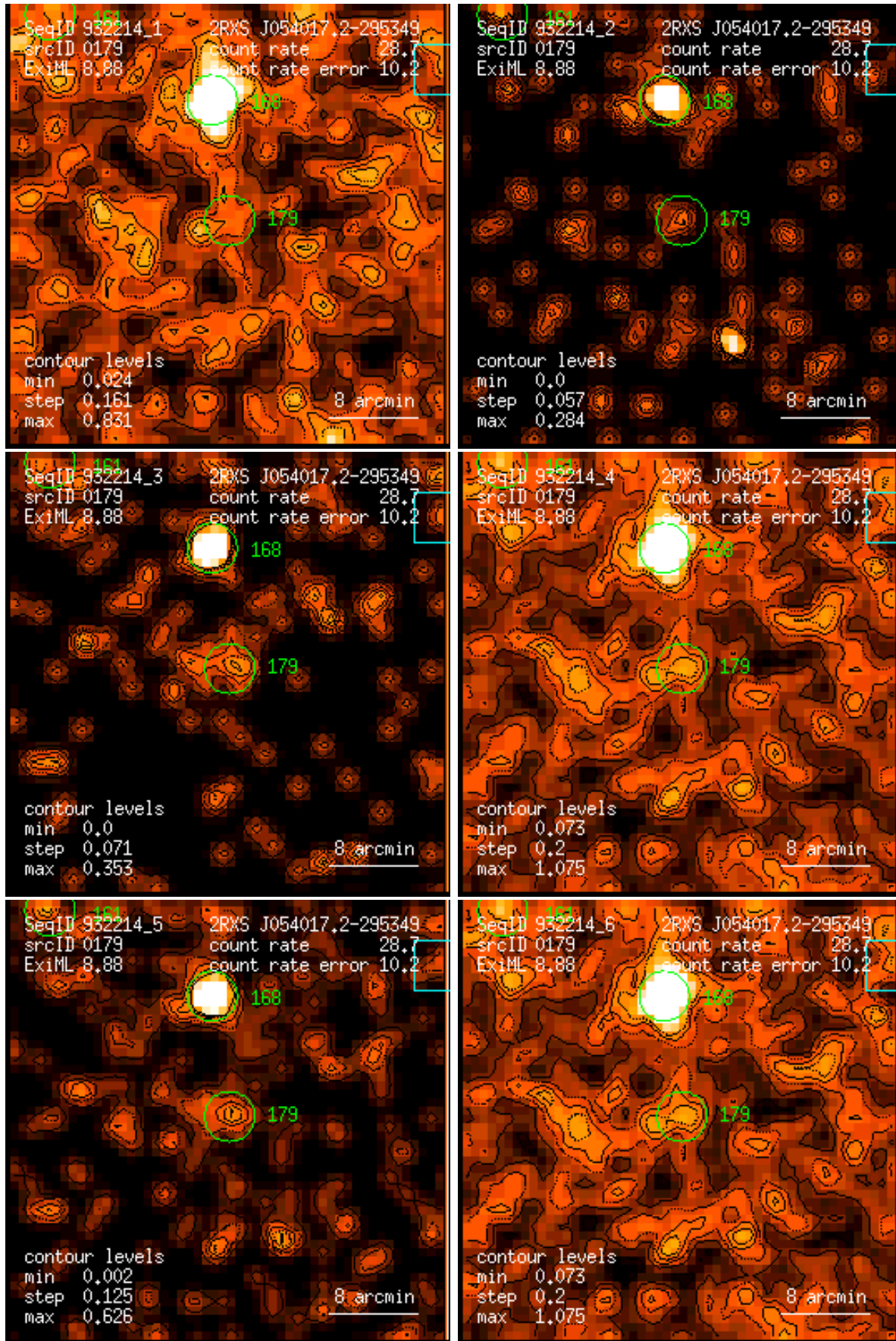
Figure 179: RASS 932214: detection 0179: band rate images, Gaussian filter: (1) PSPC channels 11 – 41, (2) 52 – 90, (3) 91 – 201, (4) 11 – 235, (5) 52 – 201, (6) 11 – 201. Broad band rates in counts/ks. Band rate contour levels in counts/ks/arcmin 2 .
