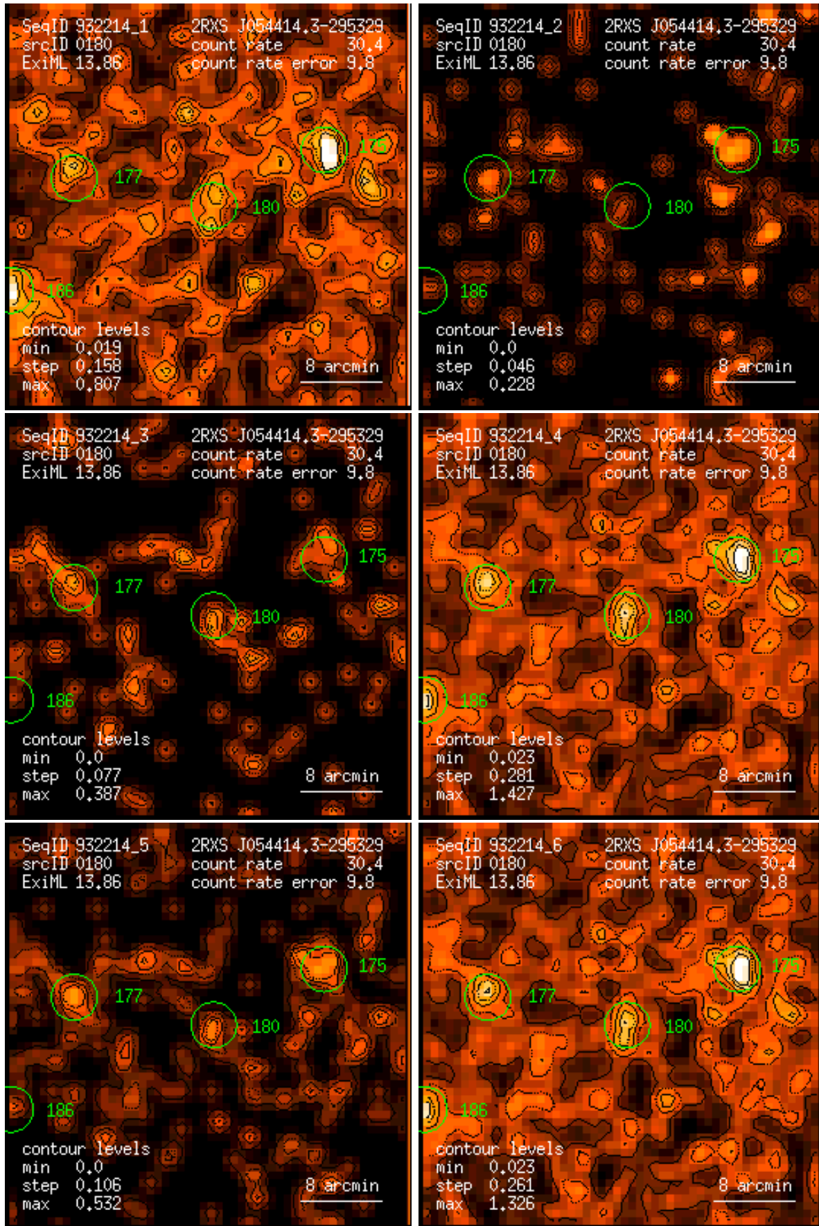
Figure 180: RASS 932214: detection 0180: band rate images, Gaussian filter: (1) PSPC channels 11 – 41, (2) 52 – 90, (3) 91 – 201, (4) 11 – 235, (5) 52 – 201, (6) 11 – 201. Broad band rates in counts/ks. Band rate contour levels in counts/ks/arcmin 2 .
