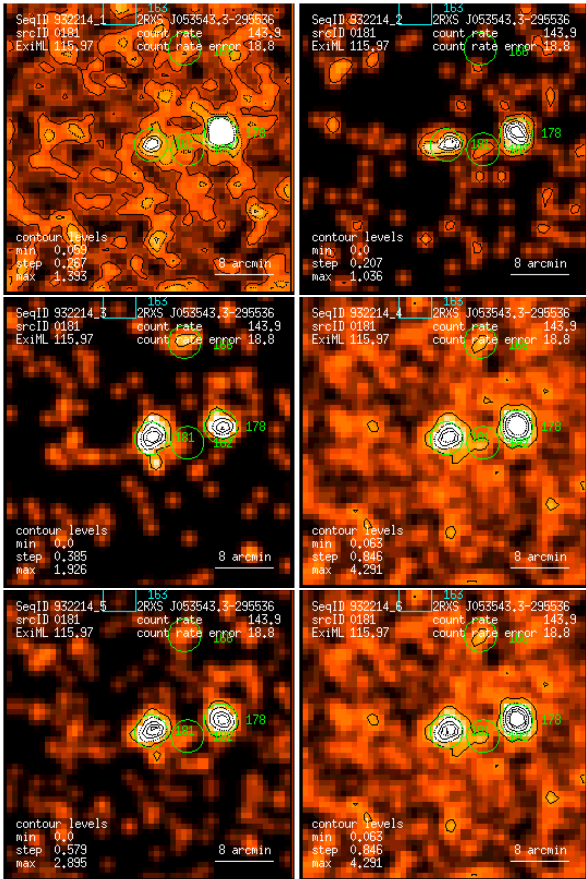
Figure 181: RASS 932214: detection 0181: band rate images, Gaussian filter: (1) PSPC channels 11 – 41, (2) 52 – 90, (3) 91 – 201, (4) 11 – 235, (5) 52 – 201, (6) 11 – 201. Broad band rates in counts/ks. Band rate contour levels in counts/ks/arcmin 2 .
