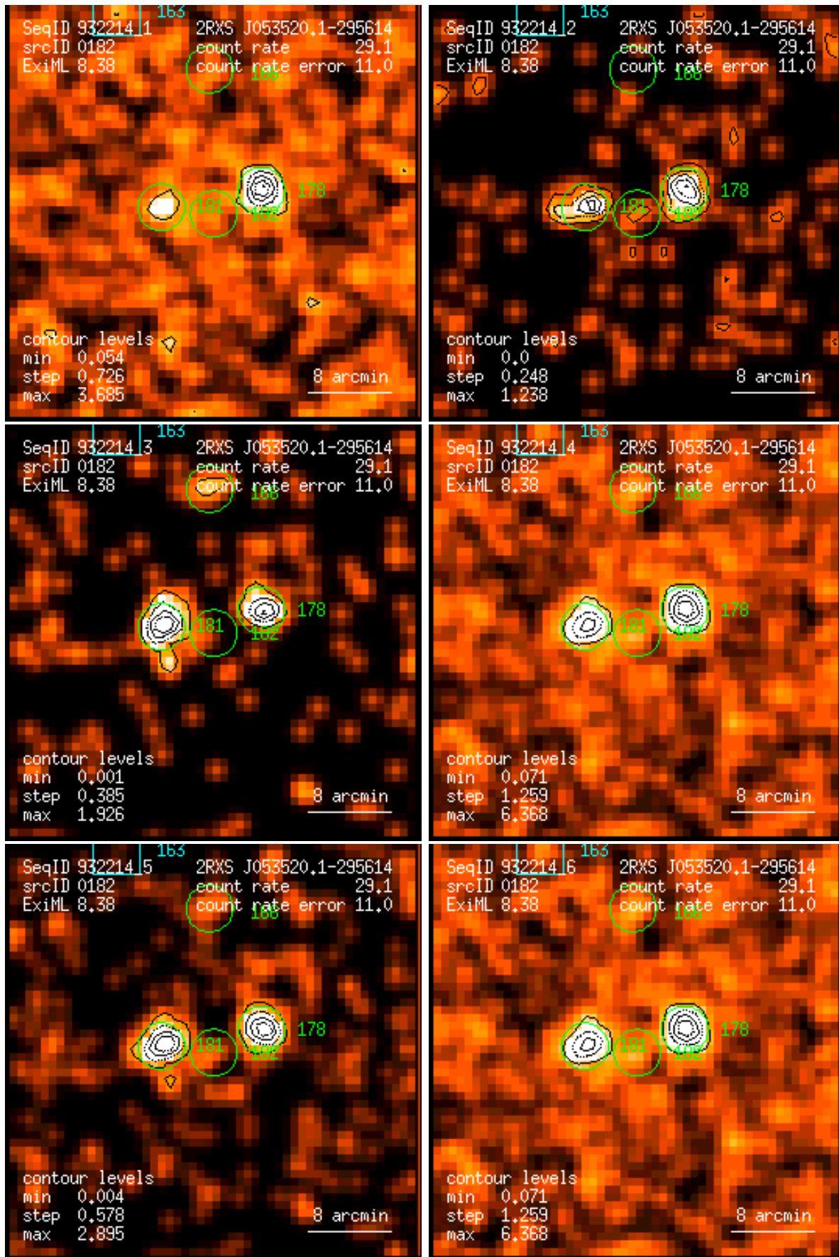
Figure 182: RASS 932214: detection 0182: band rate images, Gaussian filter: (1) PSPC channels 11 – 41, (2) 52 – 90, (3) 91 – 201, (4) 11 – 235, (5) 52 – 201, (6) 11 – 201. Broad band rates in counts/ks. Band rate contour levels in counts/ks/arcmin 2 .
