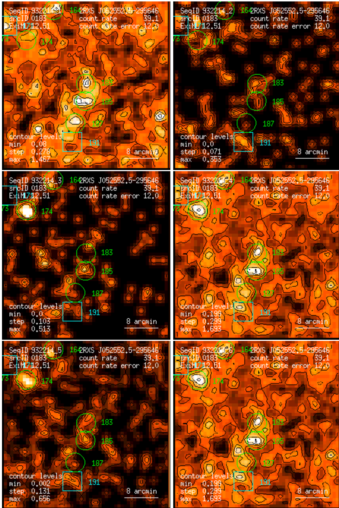
Figure 183: RASS 932214: detection 0183: band rate images, Gaussian filter: (1) PSPC channels 11 – 41, (2) 52 – 90, (3) 91 – 201, (4) 11 – 235, (5) 52 – 201, (6) 11 – 201. Broad band rates in counts/ks. Band rate contour levels in counts/ks/arcmin 2 .
