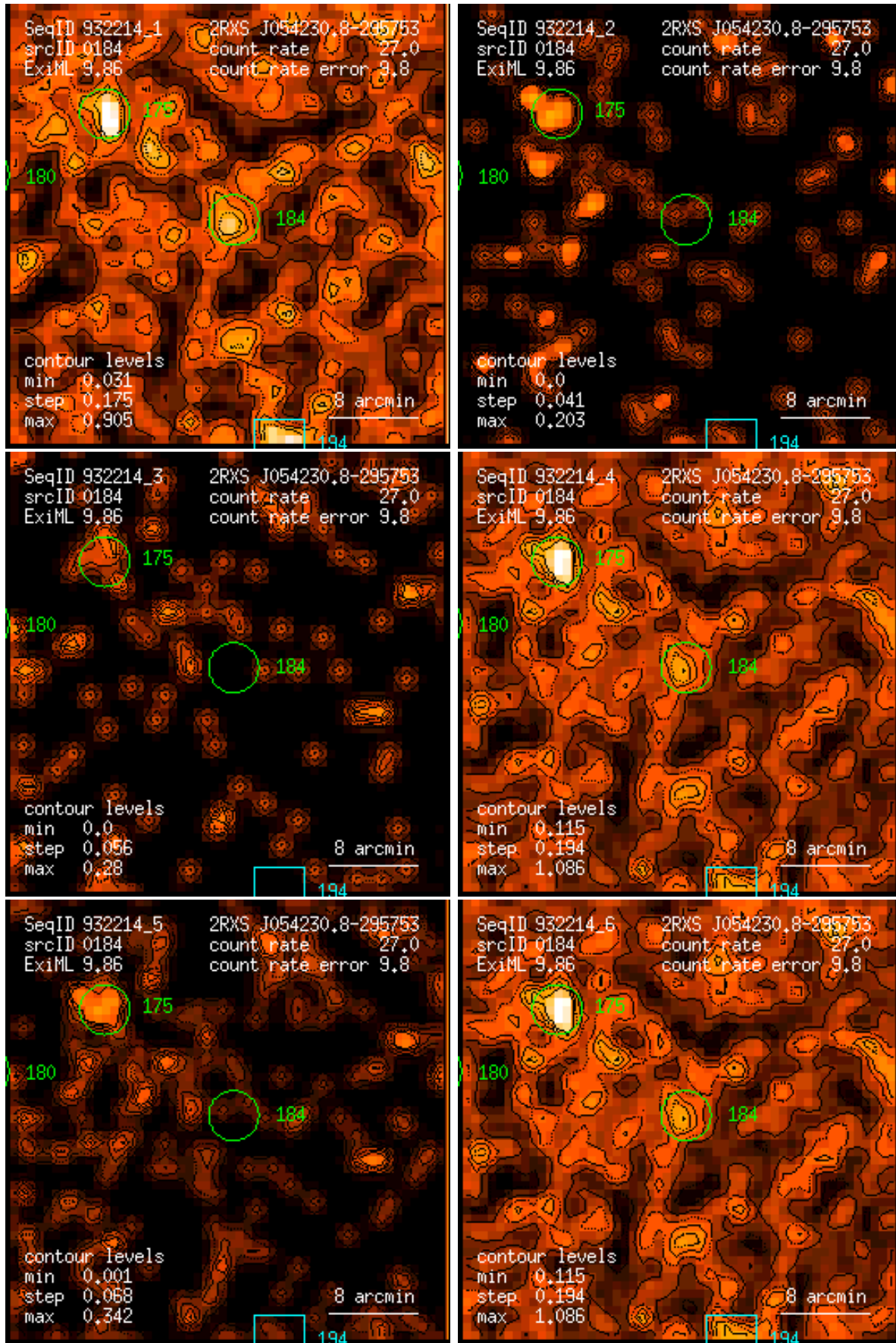
Figure 184: RASS 932214: detection 0184: band rate images, Gaussian filter: (1) PSPC channels 11 – 41, (2) 52 – 90, (3) 91 – 201, (4) 11 – 235, (5) 52 – 201, (6) 11 – 201. Broad band rates in counts/ks. Band rate contour levels in counts/ks/arcmin 2 .
