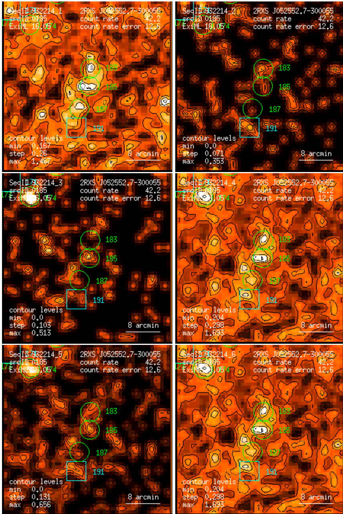
Figure 185: RASS 932214: detection 0185: band rate images, Gaussian filter: (1) PSPC channels 11 – 41, (2) 52 – 90, (3) 91 – 201, (4) 11 – 235, (5) 52 – 201, (6) 11 – 201. Broad band rates in counts/ks. Band rate contour levels in counts/ks/arcmin 2 .
