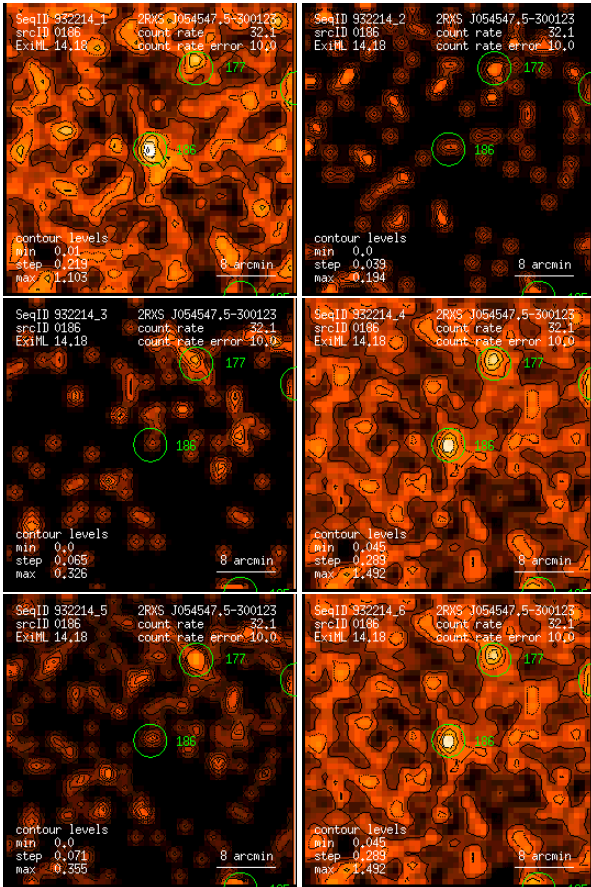
Figure 186: RASS 932214: detection 0186: band rate images, Gaussian filter: (1) PSPC channels 11 – 41, (2) 52 – 90, (3) 91 – 201, (4) 11 – 235, (5) 52 – 201, (6) 11 – 201. Broad band rates in counts/ks. Band rate contour levels in counts/ks/arcmin 2 .
