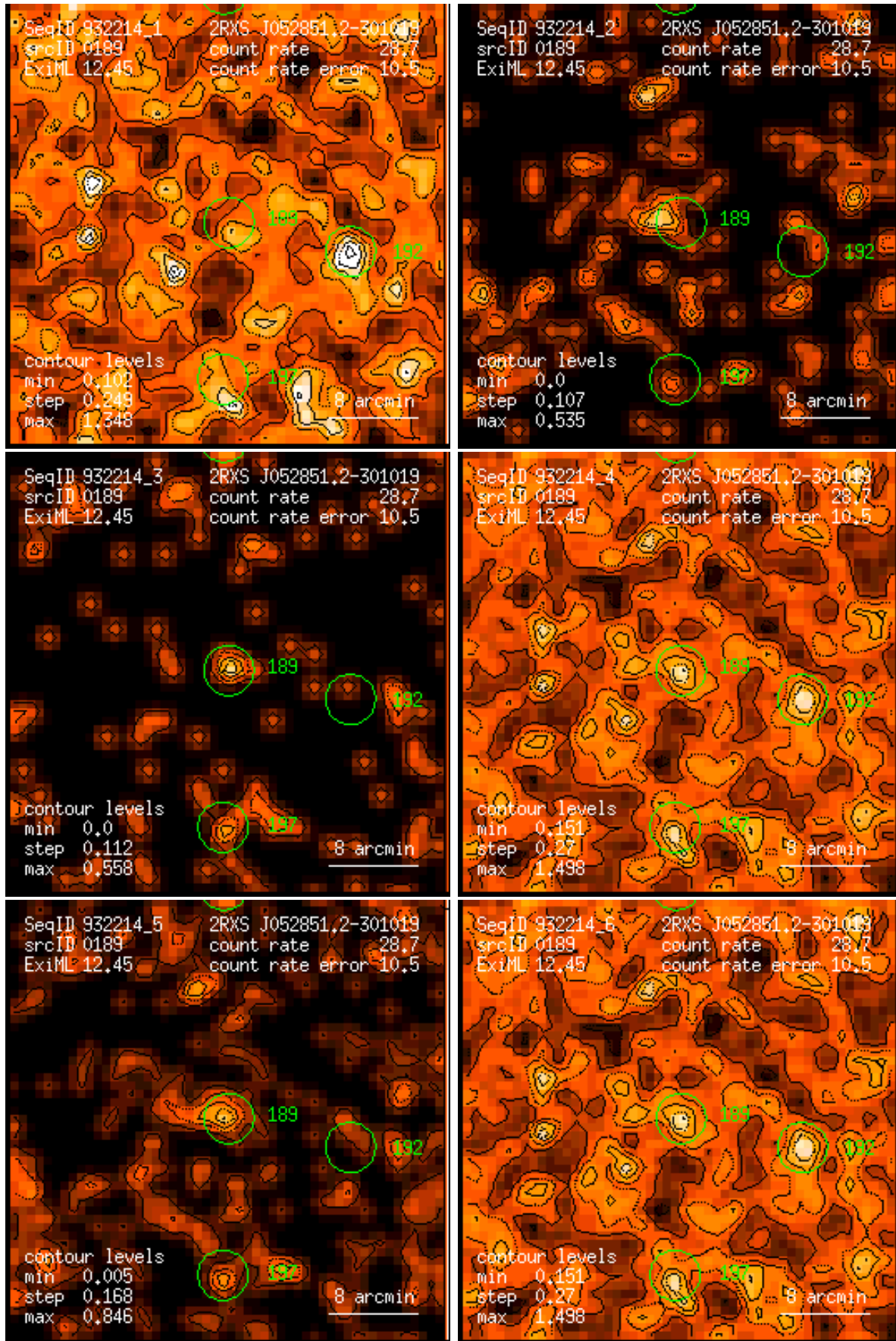
Figure 189: RASS 932214: detection 0189: band rate images, Gaussian filter: (1) PSPC channels 11 – 41, (2) 52 – 90, (3) 91 – 201, (4) 11 – 235, (5) 52 – 201, (6) 11 – 201. Broad band rates in counts/ks. Band rate contour levels in counts/ks/arcmin 2 .
