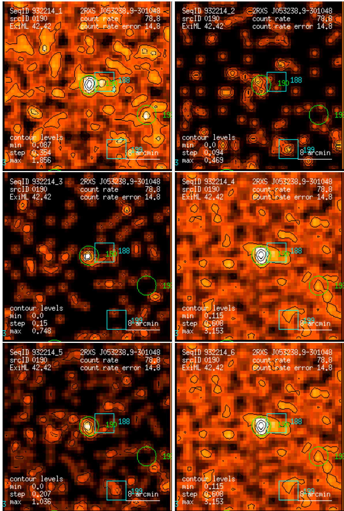
Figure 190: RASS 932214: detection 0190: band rate images, Gaussian filter: (1) PSPC channels 11 – 41, (2) 52 – 90, (3) 91 – 201, (4) 11 – 235, (5) 52 – 201, (6) 11 – 201. Broad band rates in counts/ks. Band rate contour levels in counts/ks/arcmin 2 .
