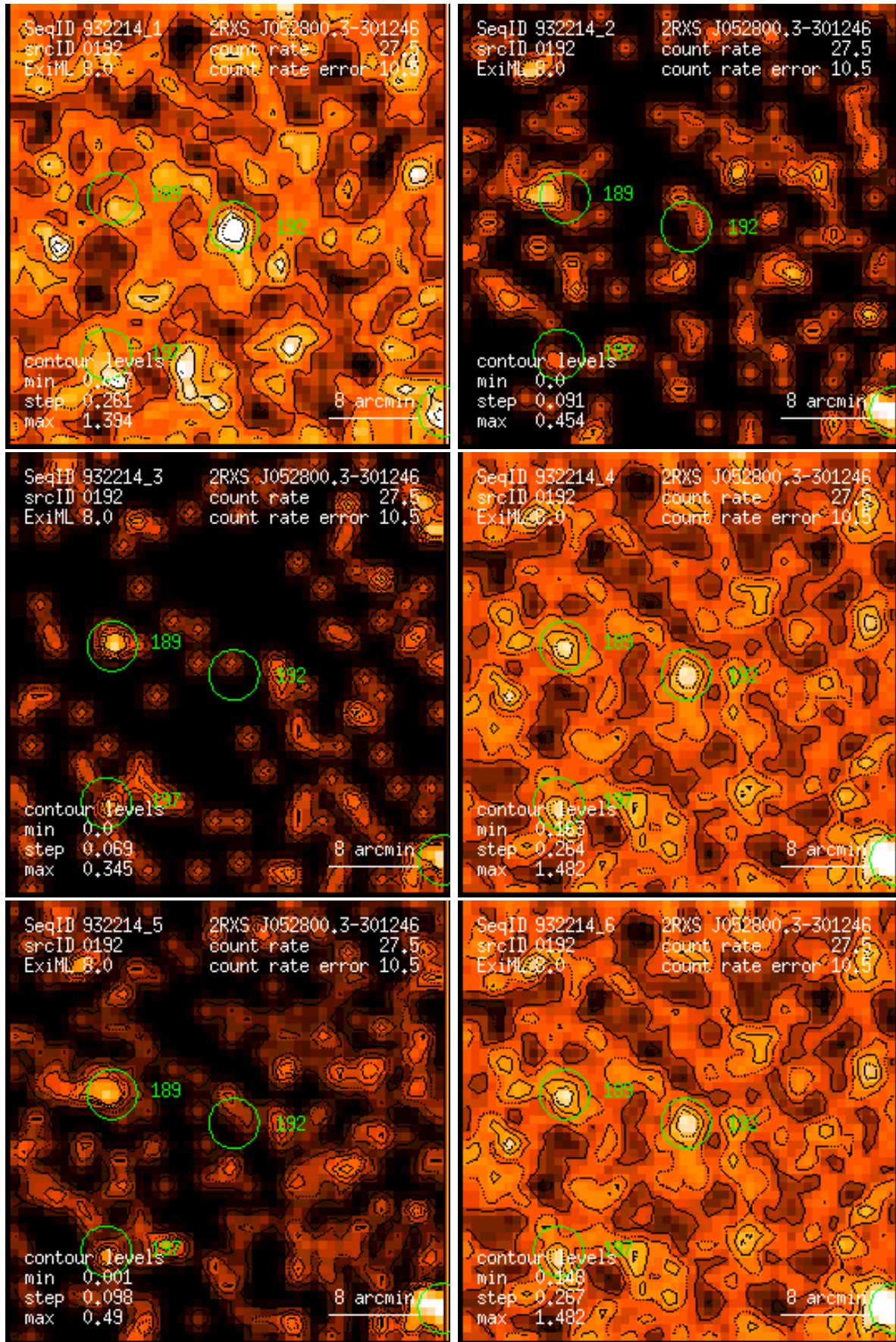
Figure 192: RASS 932214: detection 0192: band rate images, Gaussian filter: (1) PSPC channels 11 – 41, (2) 52 – 90, (3) 91 – 201, (4) 11 – 235, (5) 52 – 201, (6) 11 – 201. Broad band rates in counts/ks. Band rate contour levels in counts/ks/arcmin 2 .
