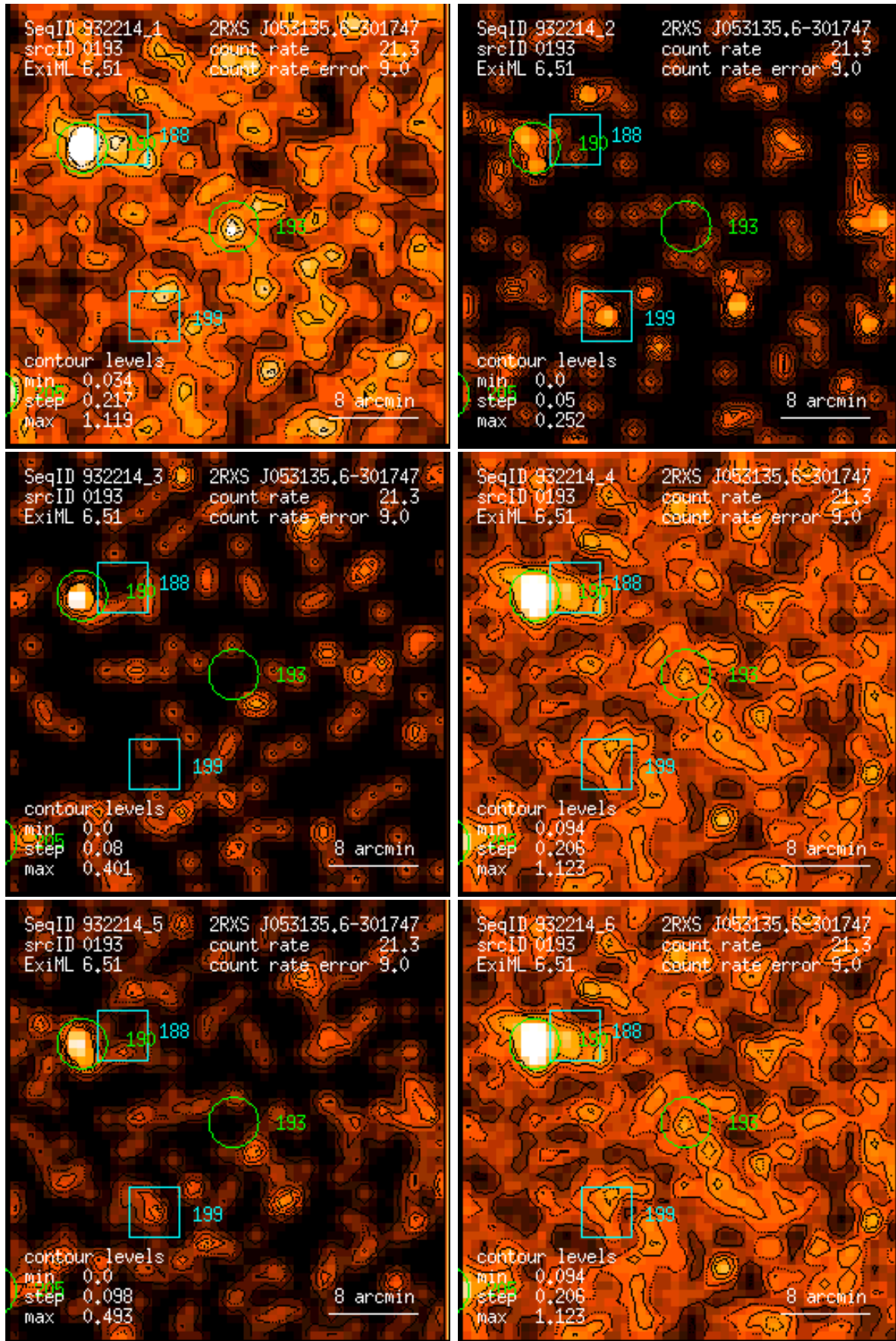
Figure 193: RASS 932214: detection 0193: band rate images, Gaussian filter: (1) PSPC channels 11 – 41, (2) 52 – 90, (3) 91 – 201, (4) 11 – 235, (5) 52 – 201, (6) 11 – 201. Broad band rates in counts/ks. Band rate contour levels in counts/ks/arcmin 2 .
