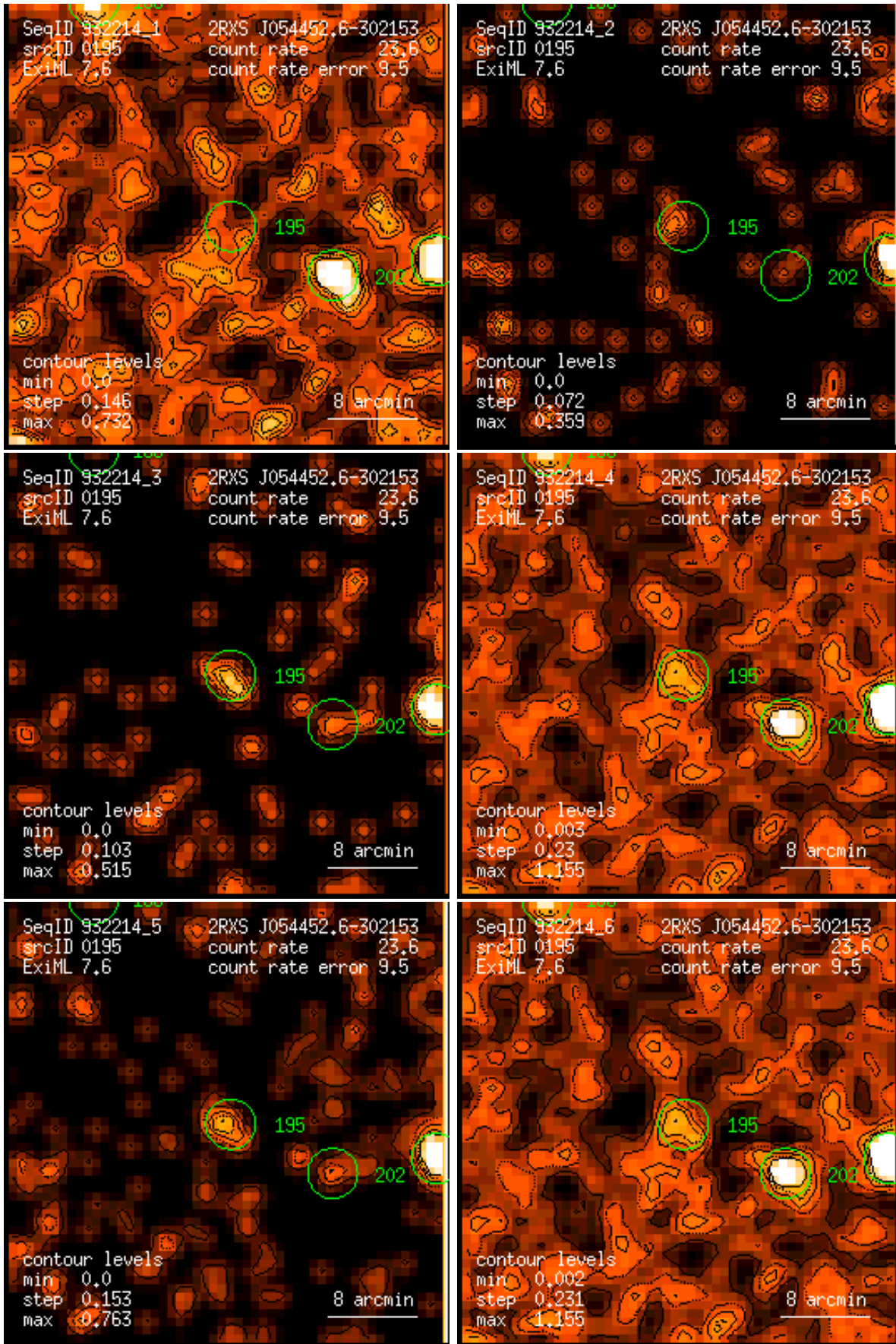
Figure 195: RASS 932214: detection 0195: band rate images, Gaussian filter: (1) PSPC channels 11 – 41, (2) 52 – 90, (3) 91 – 201, (4) 11 – 235, (5) 52 – 201, (6) 11 – 201. Broad band rates in counts/ks. Band rate contour levels in counts/ks/arcmin 2 .
