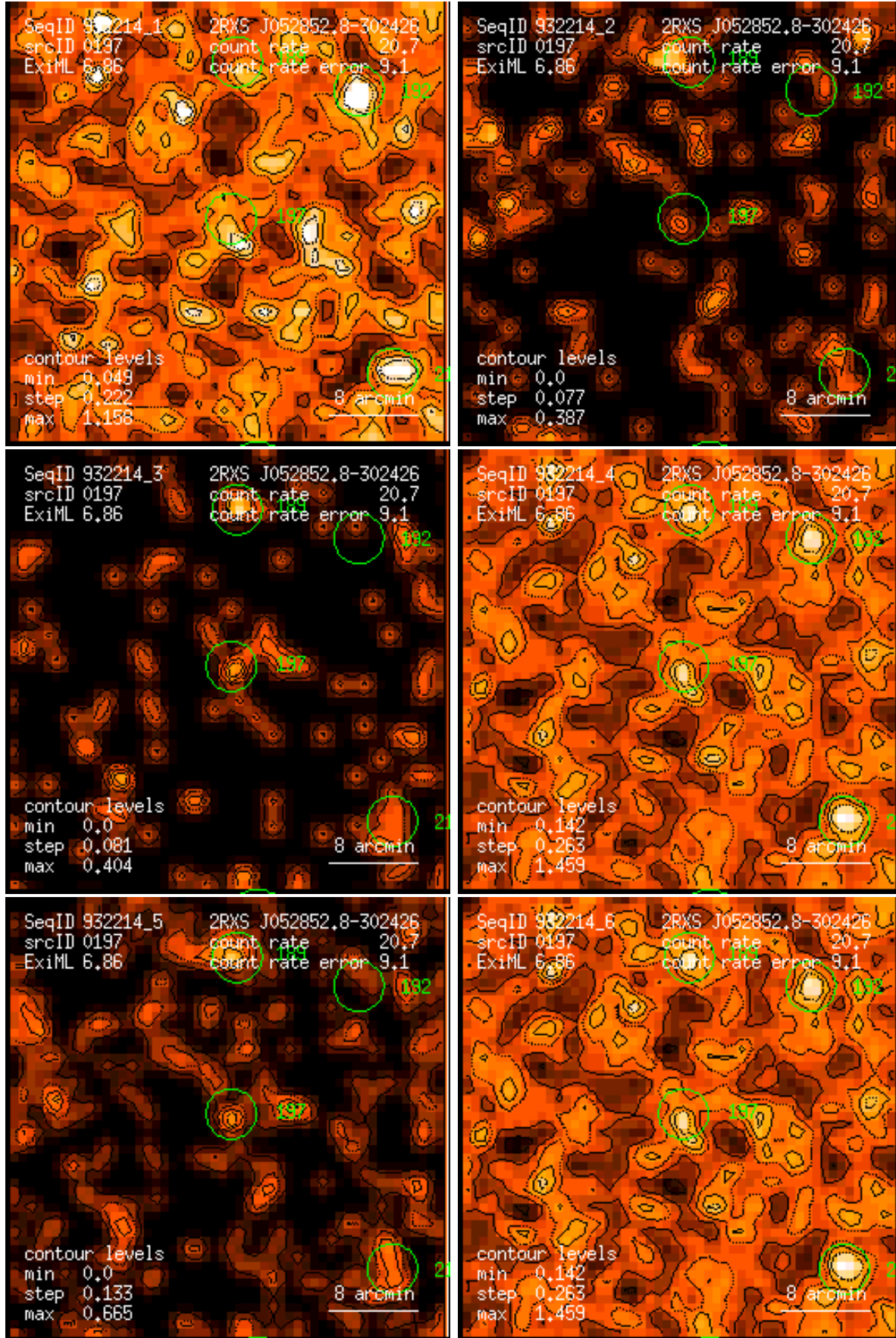
Figure 197: RASS 932214: detection 0197: band rate images, Gaussian filter: (1) PSPC channels 11 – 41, (2) 52 – 90, (3) 91 – 201, (4) 11 – 235, (5) 52 – 201, (6) 11 – 201. Broad band rates in counts/ks. Band rate contour levels in counts/ks/arcmin 2 .
