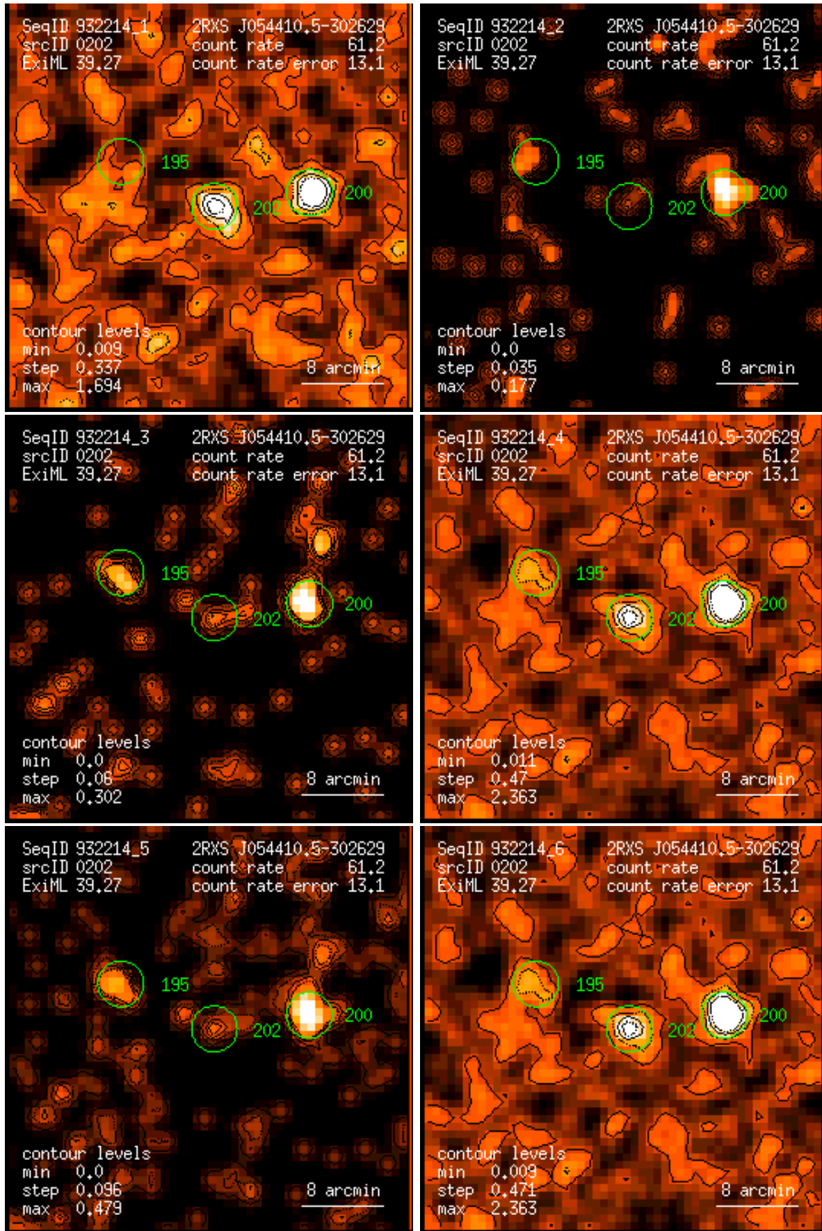
Figure 202: RASS 932214: detection 0202: band rate images, Gaussian filter: (1) PSPC channels 11 – 41, (2) 52 – 90, (3) 91 – 201, (4) 11 – 235, (5) 52 – 201, (6) 11 – 201. Broad band rates in counts/ks. Band rate contour levels in counts/ks/arcmin 2 .
