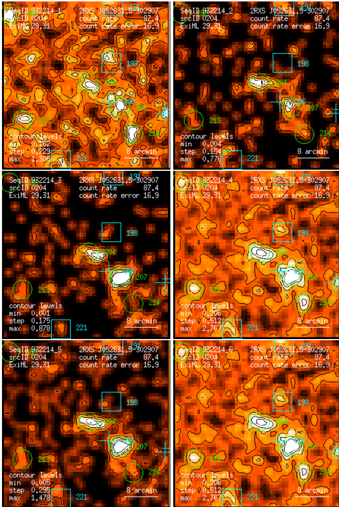
Figure 204: RASS 932214: detection 0204: band rate images, Gaussian filter: (1) PSPC channels 11 – 41, (2) 52 – 90, (3) 91 – 201, (4) 11 – 235, (5) 52 – 201, (6) 11 – 201. Broad band rates in counts/ks. Band rate contour levels in counts/ks/arcmin 2 .
