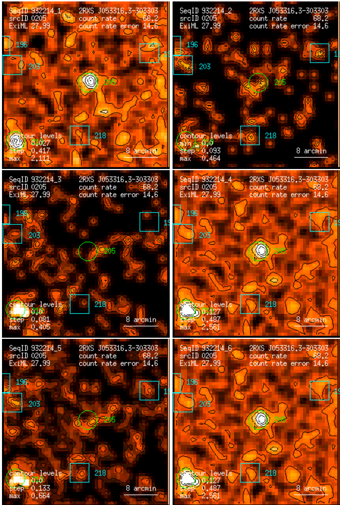
Figure 205: RASS 932214: detection 0205: band rate images, Gaussian filter: (1) PSPC channels 11 – 41, (2) 52 – 90, (3) 91 – 201, (4) 11 – 235, (5) 52 – 201, (6) 11 – 201. Broad band rates in counts/ks. Band rate contour levels in counts/ks/arcmin 2 .
