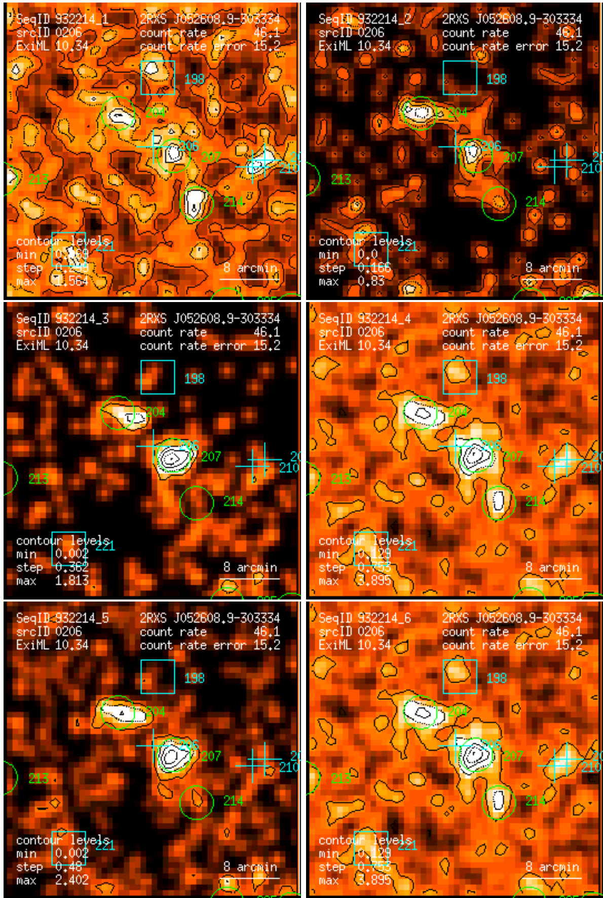
Figure 206: RASS 932214: detection 0206: band rate images, Gaussian filter: (1) PSPC channels 11 – 41, (2) 52 – 90, (3) 91 – 201, (4) 11 – 235, (5) 52 – 201, (6) 11 – 201. Broad band rates in counts/ks. Band rate contour levels in counts/ks/arcmin 2 .
